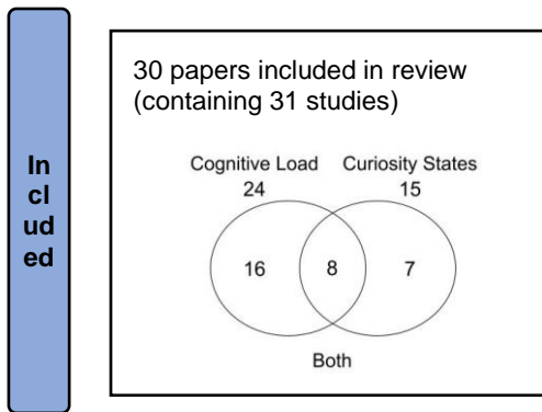
Figure 1 : PRISMA flowchart
