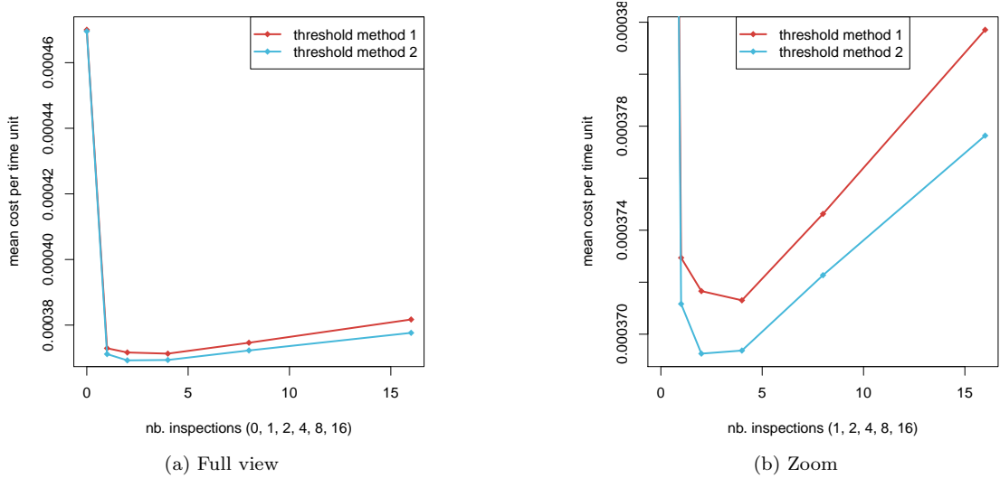
Figure 7: Cost per time unit with inspection cost, \beta = 2 , C_{Corr} = 3 , C_{Prev} = 1 , minimal repair, covariate with random effect (vs. number of inspections)
