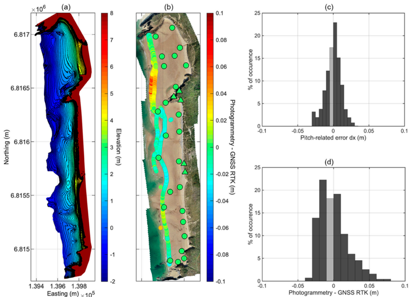
Figure 6. Quality assessment of the 0.1 m resolution photogrammetric DEM obtained using the standard workflow. (a) DEM overlapped with depth contours every 0.2 m; (b) vertical error at photogrammetric targets (GCPs and ChkPts) and 1381 RTK-GNSS survey points; (c) probability distribution function (PDF) of pitch-related error (dx) binned at 0.005 m and (d) PDF of photogrammetric vertical error in comparison to RTK-GNSS survey points binned at 0.01 m.
