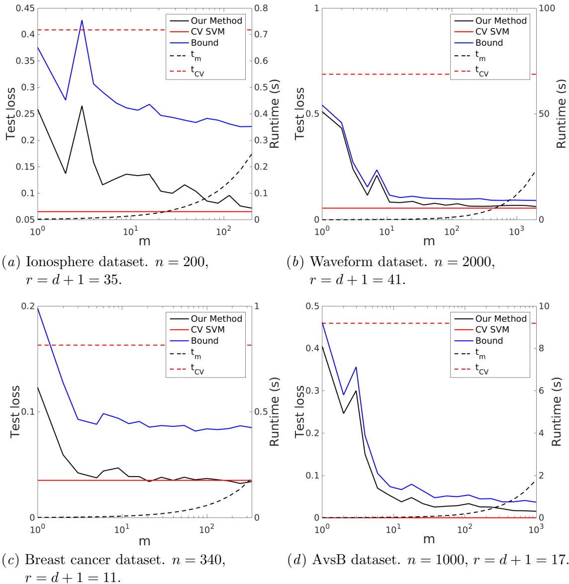
Figure 2: Comparison of PAC-Bayesian aggregation with RBF kernel SVM tuned by cross-validation. The solid red, black, and blue lines correspond, respectively, to the zero-one test loss of the cross-validated SVM, the loss of \rho -weighted majority vote, where \rho is a result of minimization of the PAC-Bayes- \lambda bound, and PAC-Bayes-kl bound on the loss of randomized classifier defined by \rho . The dashed black line represents the training time of PAC-Bayesian aggregation, while the red dashed line represents the training time of cross-validated SVM. The prediction accuracy and run time of PAC-Bayesian aggregation and PAC-Bayes-kl bound are given as functions of the hypothesis set size m .
