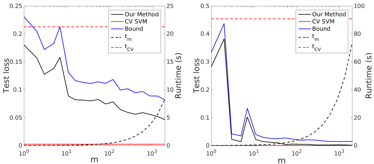
(c) Skin dataset. n = 2000 , r = \sqrt{n} = 45 . (d) Mushrooms dataset. n = 2000 , r = d + 1 = 113 .
