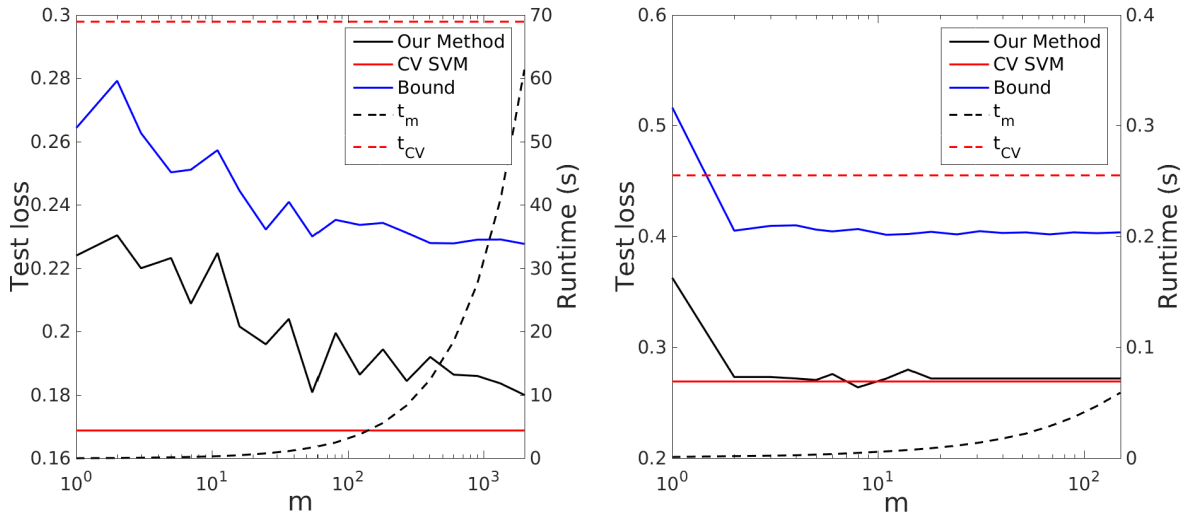
(a) Adult dataset. n = 2000 , r = d + 1 = 123 . (b) Haberman dataset. n = 150 , r = \sqrt{n} = 12 .
