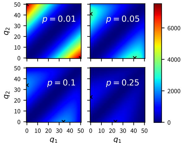
Fig. 12: Upper bound (116) on the quantum Fisher information of a superposition of two Dicke states on n = 50 spin-1/2 particles after being exposed to i.i.d. amplitude-damping noise. A Dicke state with q excitations is an even superposition of all states with exactly q excitations. For each q_1, q_2 , the considered state is an even superposition of the two Dicke states with a number q_1 and q_2 of downwards-pointing spins respectively. Each plot corresponds to a different value of the single-site amplitude-damping noise parameter p . Our bound attains its maximum on this family of states (black crosses) for states that are an even superposition of the highest excited state and of a weakly excited Dicke state that is separated from the ground state. This separation hinders Eve from accurately guessing the energy of Alice's state, which via our trade-off relation improves the state's sensitivity after application of the noisy channel. The bound is computed with k = n = 50 .
