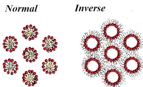
Figure 7 - Cross-section of the normal and inverse (or reverse) Hexagonal phase (heads in red, tails in grey).
