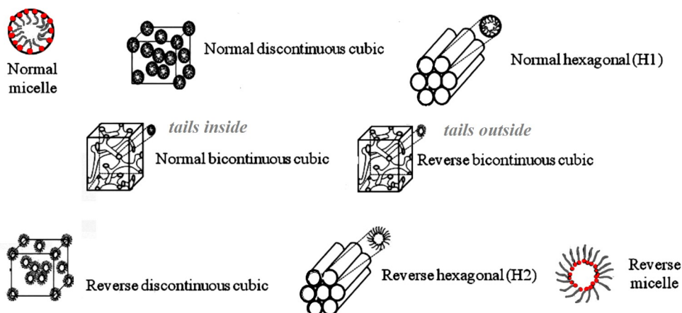
Figure 10: Some normal and reverse phases, as illustrated by Huang and Gui (2018), in an article released according to CC BY-NC 4.0. Many thanks to the authors.
