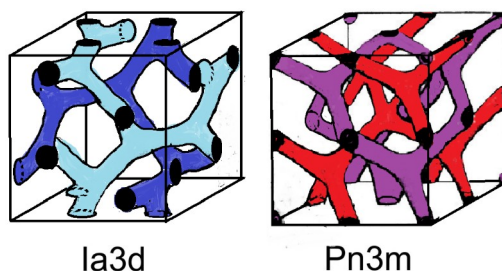
Figure 9: Ia3d compared with Pn3m , as depicted by Tresset, 2009.
