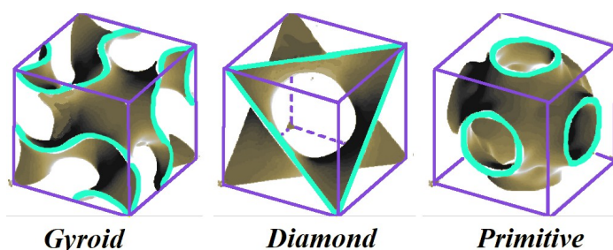
Figure 11: For this illustration, we used the view of the surfaces given in the Figure 1 of the article by Yagmur et al., 2007 (many thanks to the authors). The P-, D- and G-surfaces are linked by a Bonnet transformation (Lidin, 1990),
