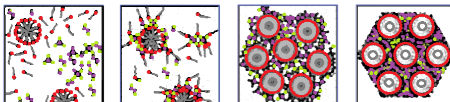
Figure 2: Here a cartoon according to that proposed by Wan and Zhao to illustrate the pathway A. From left to right: liquid solution with micelles, surfactant molecules (red heads and gray tails) and inorganic species (violet and green); micelles surrounded by the inorganic species; micelles arranged in a quasi-hexagonal geometry; condensation of inorganic silica around the surfactant.
