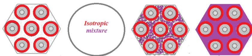
Figure 4: In the pathway given by Attard et al. and by Bruchner et al., the hexagonal inorganic-organic mixture is coming from an isotropic mixture, observed after the silica precursor is added to the LLC. From left to right: liquid crystal in the Type I Hexagonal phase; isotropic mixture; inorganic species (violet) in the water surrounding the micelles; condensation of inorganic silica around the surfactant.
