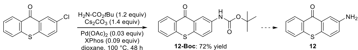
Scheme 4. Alternative route to (Boc-protected) 2-aminothioxanthone ( 12 ).
