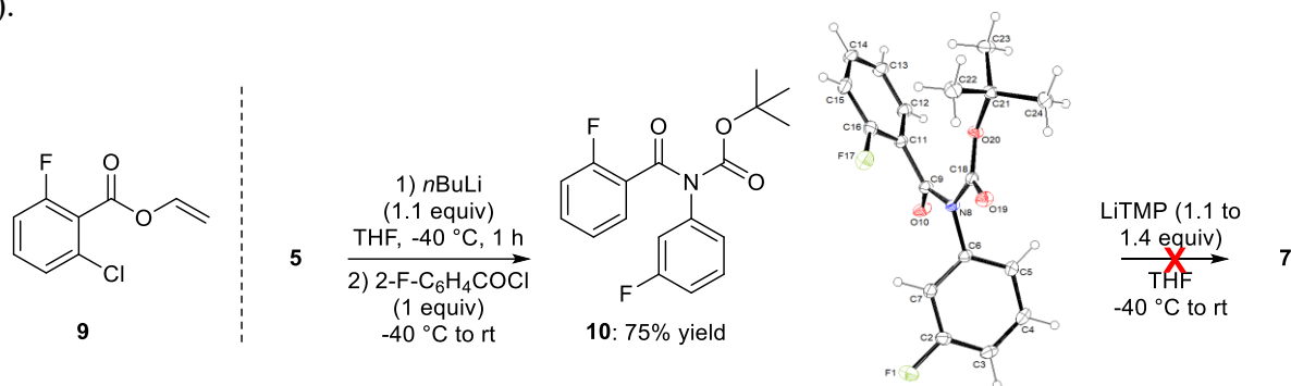
Scheme 2. Left: Example of a vinyl ester obtained as a side product using an acyl chloride to intercept an aryllithium prepared in THF. Right: Attempted rearrangement of tert -butyl N -(2-fluorobenzoyl)- N -(3-fluorophenyl)carbamate ( 10 ) and ORTEP diagram (30% probability) of 10 .
