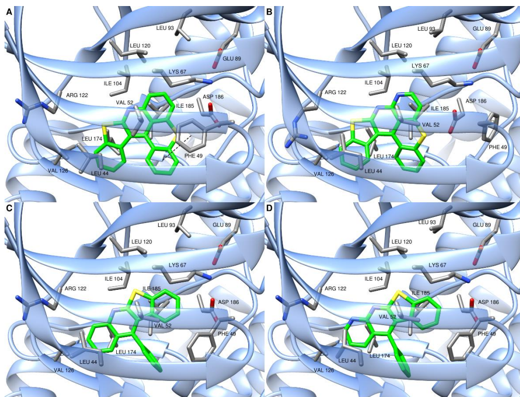
Figure 4. Plausible binding mode of MN34-20 (A), 39 (B), NM-049 (C) and NM65-45 (D) within PIM1 ATP-binding site. The images were produced using UCSF Chimera. 77
