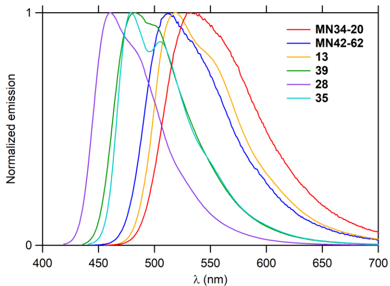
Figure 7. Emission spectra of the hexacycles in toluene.
