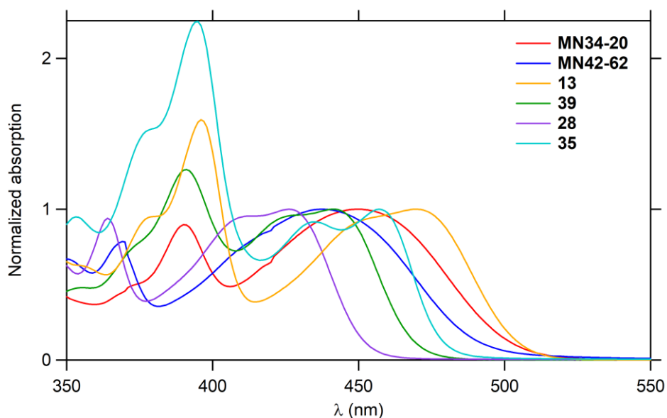
Figure 6. Absorption spectra of the hexacycles in toluene.
