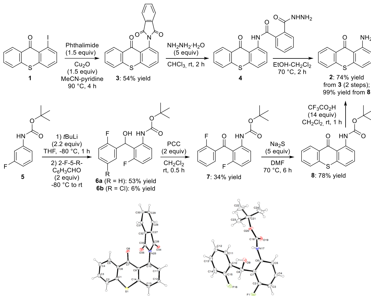
Scheme 1. Alternative routes to 1-aminothioxanthone ( 2 ) and ORTEP diagrams (30% probability) of the compounds 3 and 6a .
