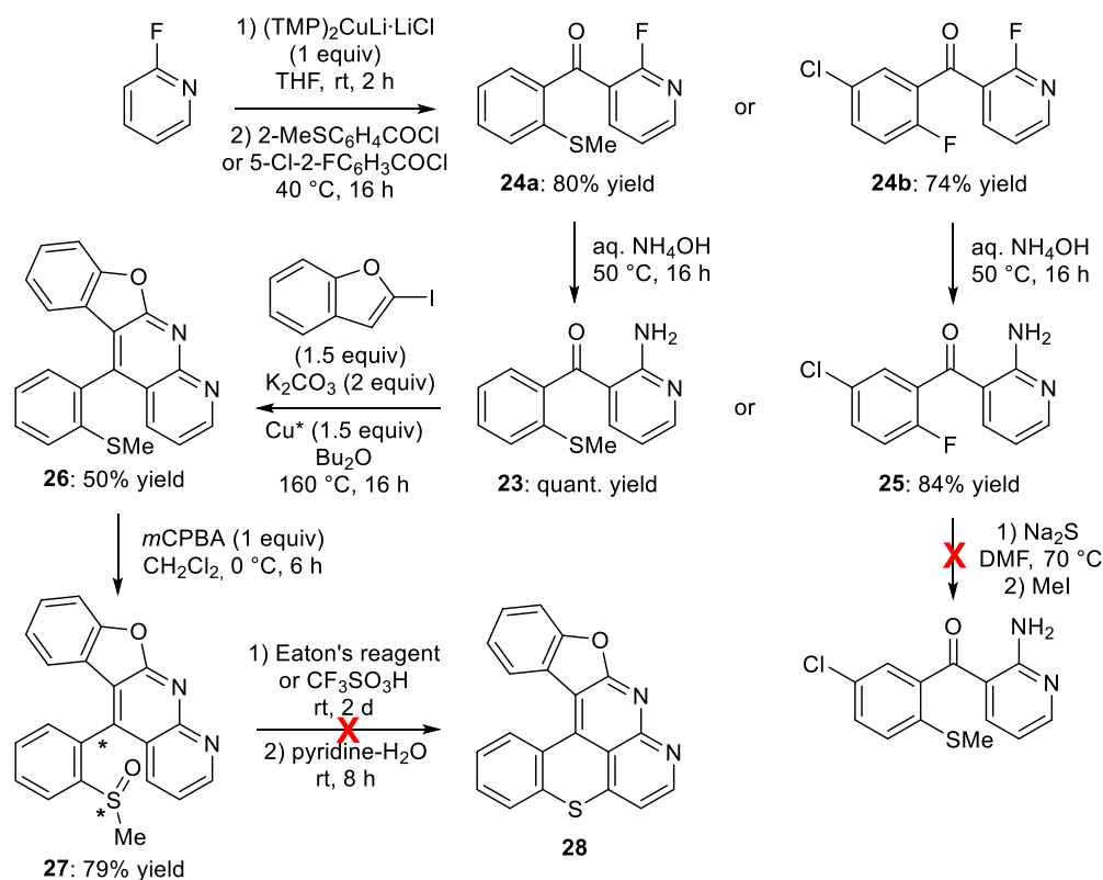
Scheme 8. Unsuccessful attempt toward benzofuro[2,3- b ]benzothiopyrano[4,3,2- de ]1,8-naphthyridine ( 28 ).
