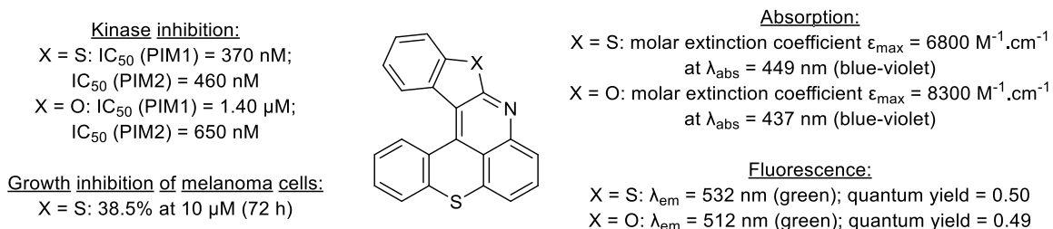
Figure 1. Properties of benzothieno[2,3- b ]benzothiopyrano[4,3,2- de ]quinoline ( MN34-20 ; X = S) and benzofuro[2,3- b ]benzothiopyrano[4,3,2- de ]quinoline ( MN42-62 ; X = O).
