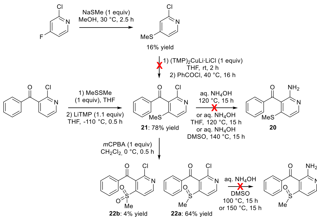
Scheme 7. Unsuccessful attempts toward 2-amino-3-benzoyl-4-(methylthio)pyridine ( 20 ) and 2-amino-3-benzoyl-4-(methylsulfinyl)pyridine.
