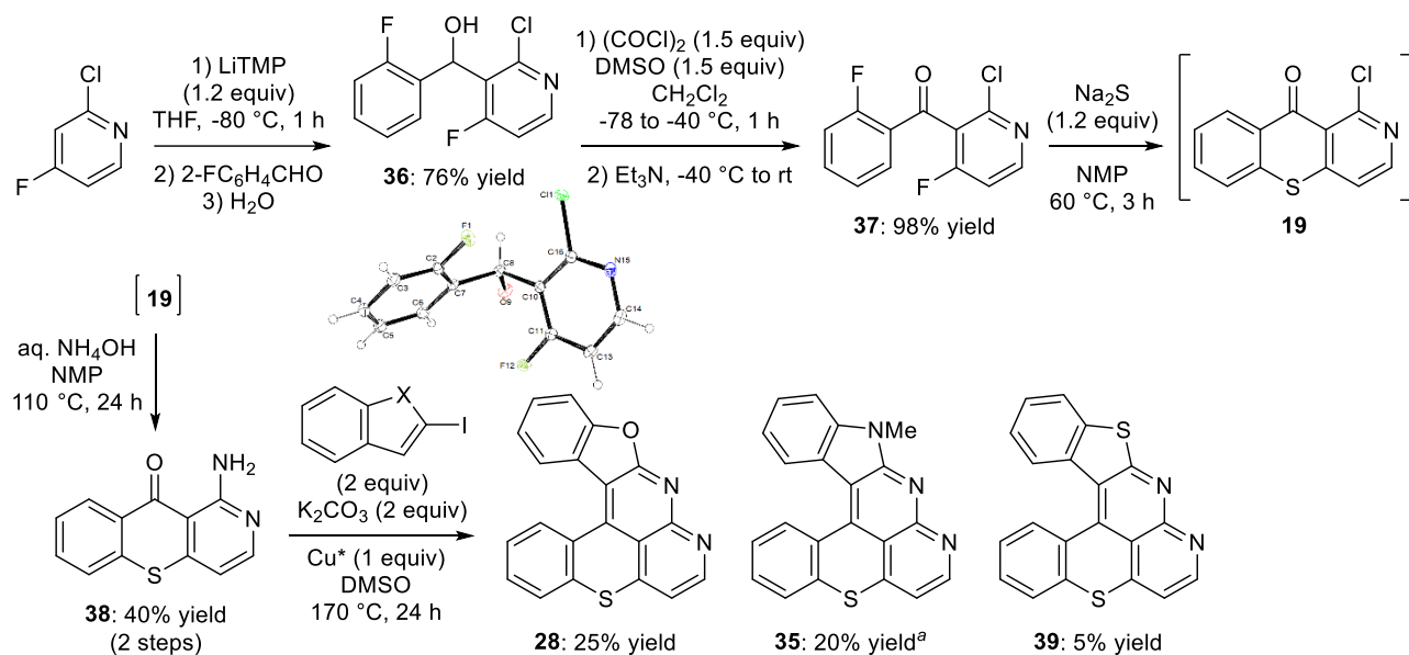
Scheme 10. Synthesis of benzofuro[2,3- b ]benzothiopyrano[4,3,2- de ]1,8-naphthyridine ( 28 ), 10-methylbenzothiopyrano[4,3,2- de ]indolo[2,3- b ]1,8-naphthyridine ( 35 ) and benzothieno[2,3- b ]benzothiopyrano[4,3,2- de ]1,8-naphthyridine ( 39 ), and ORTEP diagram (30% probability) of the compound 36 . a 0.2 equiv of activated copper (Cu*) was used in this case.
