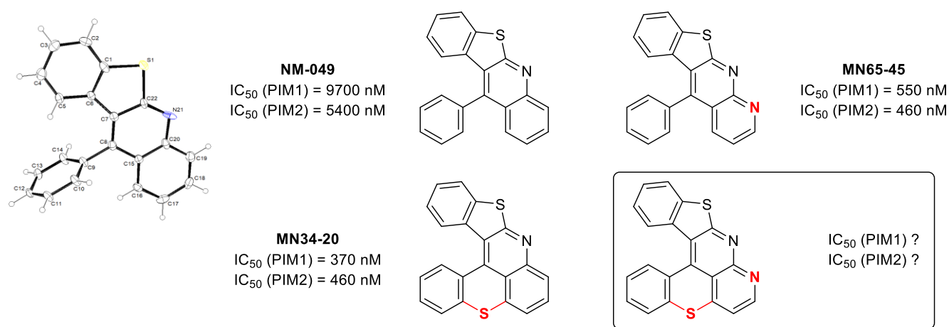
Figure 2. Structure-activity relationships leading to benzothieno[2,3- b ]benzothiopyrano[4,3,2- de ]1,8-naphthyridine, and ORTEP diagram (30% probability) of the compound NM-049 .
