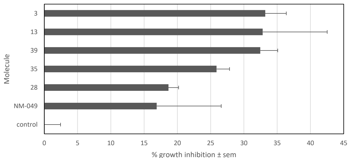
Figure 5. Antiproliferative activity (% growth inhibition) of the compounds 3 , 13 , 28 , 35 , 39 and NM-049 . 2000 A2058 human melanoma cells were treated for 72 h with 10^{-5} M of compound. Control cells were treated with an equivalent dose of DMSO (solvent of the tested compounds).
