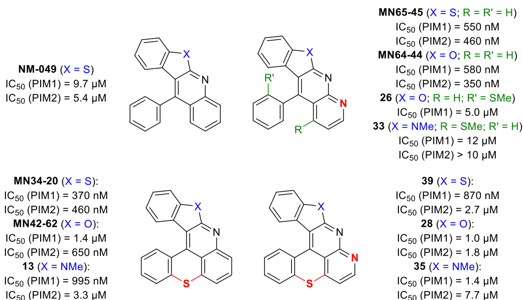
Figure 3. IC_{50} values for some of the synthesized products and related compounds. ATP concentration used in the kinase assays was 10 \mu M.
