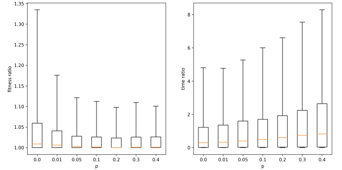
Fig. 8: The ratio of the best fitness (left) and the run time (right) of the SAP-EA with \mu = 1 , \alpha = 0.4 , \beta = 35 , and different values of p compared to the SAP-B. The run times of SAP-B range from 0.3 seconds to 30 minutes, with better time ratios for higher SAP-B run times. Each boxplot contains the data of all 20 runs per value of k and per each of the 25 scenarios, totaling to 2000 points per box. The orange line depicts the median, the box the mid-50% of the data, and the whiskers the mid 95%. A higher value of p , i.e., an increased use of RandomPwD, yields generally better solutions and a smaller spread but also increases the run time. A sweet spot seems to be around p = 0.05 . Please also refer to Section V-B2.
