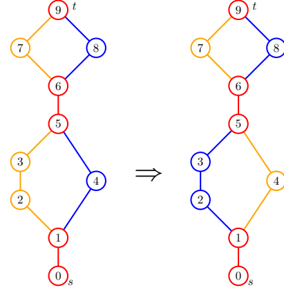
Fig. 9: An example for the ExSegment operator (Section III-B4). In this case, s = v_0 , t = v_9 , and the two paths are visualized in orange and blue, respectively, with their shared sections in red (left). After removing the cycles, only the red parts remain, leading to the set of divergence points v_1 and v_6 , while the goto points are v_5 and v_9 . Choosing randomly from the divergence points, and then from the set of goto points coming after the chosen point, this choice could be v_1 and v_5 . The two paths swap their road segments between the chosen points, visualized on the right.
