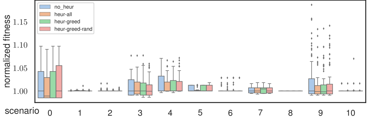
Fig. 6: Boxplots (Section IV-B) of the normalized best fitness of the MREA after 150 iterations for the 11 scenarios, with 75 runs per scenario. Each of the four colors, from left to right, represents one different crossover operator (including no crossover). Per scenario, the fitness is normalized to the median of no_heur . The configuration heur-all performs best, but only slightly. There is no clear difference between heur-greed and heur-greed-rand . In general, using crossover reduces the spread of the results. Please refer to Section IV-E for more details.
