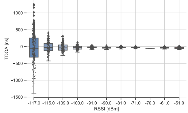
Fig. 1. TDOA values versus RSS for DR=5
