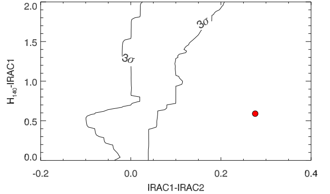
Fig. 1. Two color diagram to separate stars and galaxies. The 3\sigma external locus of the modeled star distribution is shown by a black contour, the unresolved object from our sample is shown in red, and is most probably extragalactic.
