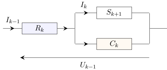
FIGURE 2. Recurrent pattern of RC circuit
