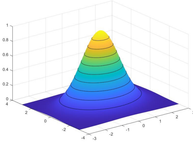
FIGURE 4. Elementary approximation of a Gaussian function
