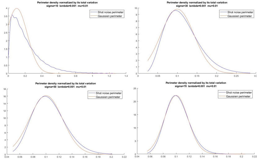
FIGURE 10. Gaussian and shot noise perimeter computed with (25) and Algorithm 2. The parameters are \lambda = 0.001 , \mu = \frac{1}{100} and from top left to bottom right \sigma = 10, 30, 50, 70 .
