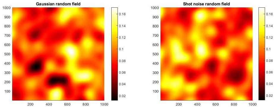
FIGURE 8. Gaussian and shot noise random fields simulated on T = [0, 1000]^2 with \lambda = 0.001 , \mu = \frac{1}{100} and \sigma = 50 .
