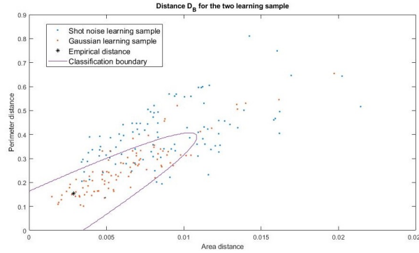
FIGURE 3. Example of a classification, with the two learning samples of size N = 50 and the classification boundary. The initial Gaussian field B was simulated using \lambda = 0.001 , \mu = 0.01 and \sigma = 50 .
