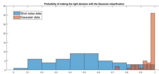
FIGURE 9. Results for the Gaussian classification. In red, a histogram of the classifications score (S_1^B(d^B(f_{1,j})))_j obtained from a sample of M = 50 initial Gaussian fields. In blue, the score (S_2^B(d^B(f_{2,j})))_j for M = 50 shot noise fields.
