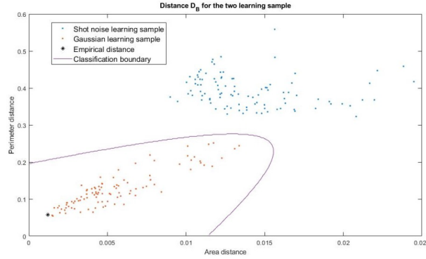
FIGURE 2. Example of a classification, with the two learning samples of size N = 50 and the classification boundary. The initial Gaussian field B was simulated using \lambda = 0.001 , \mu = 0.01 and \sigma = 30 .
