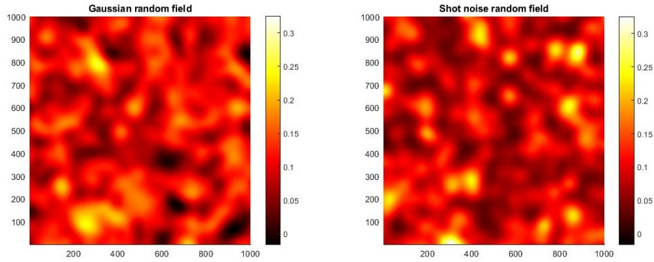
FIGURE 7. Gaussian and shot noise random fields simulated on T = [0, 1000]^2 with \lambda = 0.001 , \mu = \frac{1}{100} and \sigma = 30 .
