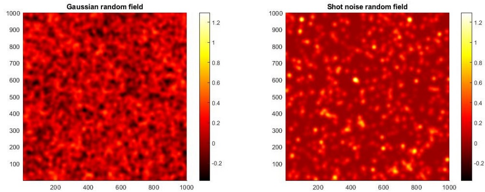
FIGURE 6. Gaussian and shot noise random fields simulated on T = [0, 1000]^2 with \lambda = 0.001 , \mu = \frac{1}{100} and \sigma = 10 .
