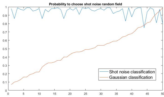
FIGURE 13. The two scores S_2^B(d^B(f_{2,j}))_j and S_2^X(d^X(f_{2,j}))_j for a sample of size 50 of initial shot noise random field f .
