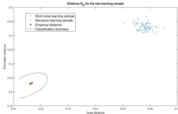
FIGURE 1. Example of a classification, with the two learning samples of size N = 50 and the classification boundary. The initial Gaussian field B was simulated using \lambda = 0.001 , \mu = 0.01 and \sigma = 10 .
