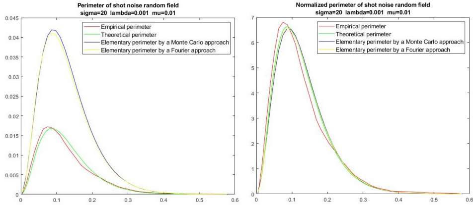
FIGURE 5. Perimeter and normalized perimeter of a Gaussian shot noise random field with exponential marks. The parameters are in the title. In red, the empirical perimeter from a simulation on F = [0, 1000]^2 and in green its theoretical formula u \mapsto \overline{\text{Per}(E_X(u))} approximated by Algorithm 1. In blue and yellow, the elementary asymptotic perimeter u \mapsto \overline{\overline{\text{Per}(E_X(u))}} approximated by Algorithm 3 and 2.
