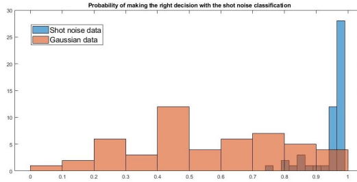
FIGURE 11. Results for the shot noise classification. In red, a histogram of the classifications score (S_1^X(d^X(f_{1,j})))_j obtained from a sample of M = 50 initial Gaussian fields. In blue, the score (S_2^X(d^X(f_{2,j})))_j for a sample of M = 50 shot noise fields. The samples are the same as in Figure 9.
