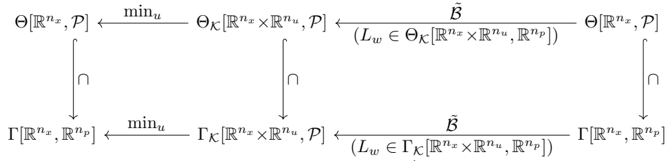
Figure 1: Stability of the classes of functions \Theta and \Gamma by the Bellman operator \mathcal{B} .
