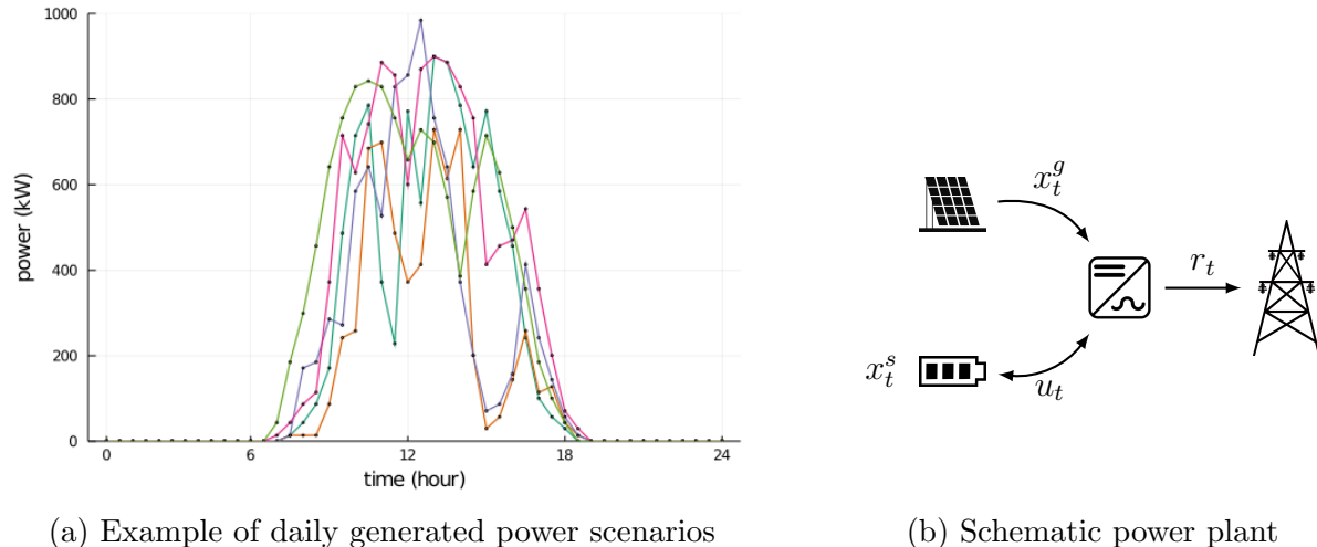
Figure 2: Description of the solar power plant: (a) examples of daily generated power scenarios (data from [1]) and (b) schematic organization
