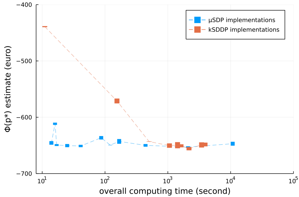
Figure 3: Estimate of \Phi(p^*) \in [\underline{V}_0(x_0), \overline{V}_0(x_0)] in (39) (marker span on the Y -axis) for implementations of \mu SDP (in blue) and k SDDP (in orange); and overall computing time for the computation of p^* ( X -axis in log scale). For both axis, the lower the values the better
