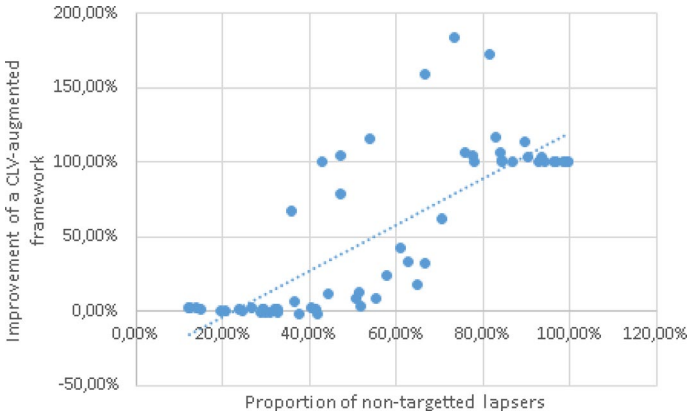
Fig. 24 Correlation between the proportion of non-targetted lapsers and the improvement of a CLV-augmented LMS.(Taking the results of XGBoost and excluding LMS n°B-27 that has a very high improvement ratio.)
