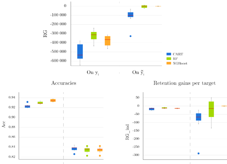
Fig. 3 Strategy no A-5: (Very negative result on y_i and a loss-limiting result on \tilde{y}_i )
