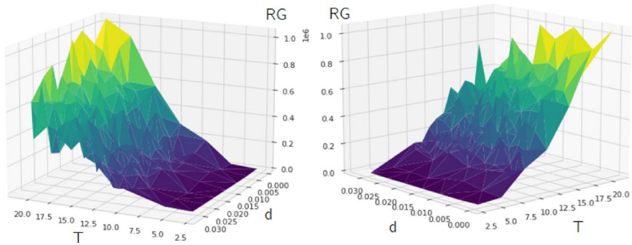
Fig. 8 3d plot ( d , T , RG )
