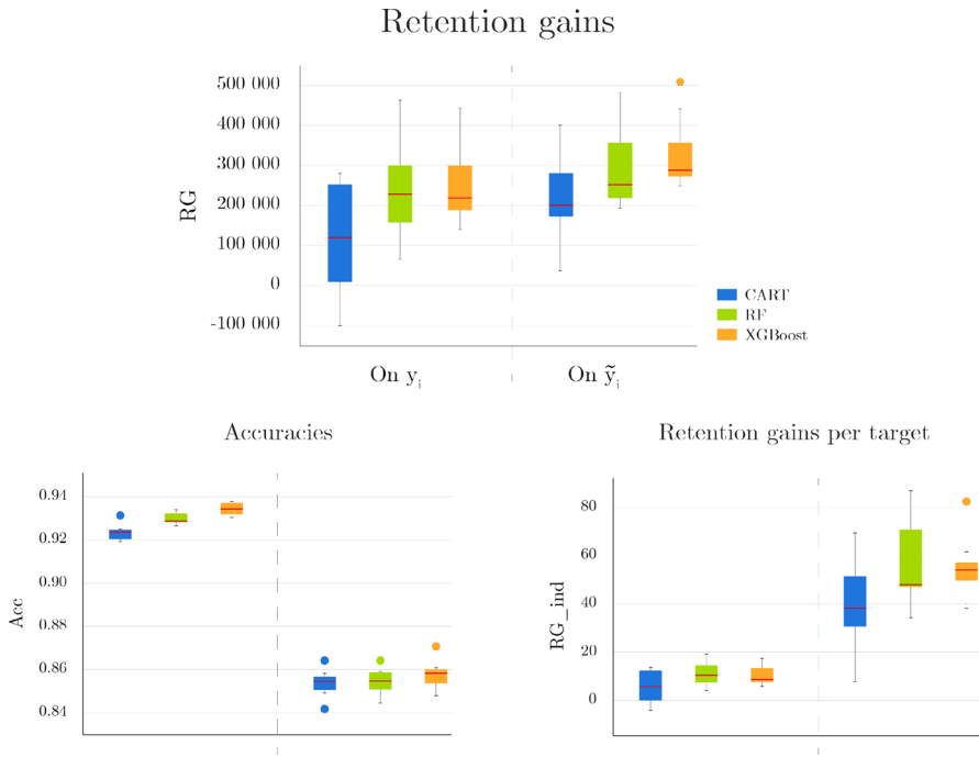
Fig. 2 Strategy no A-1: (Positive result on y_i and an improved result on \hat{y}_i )
