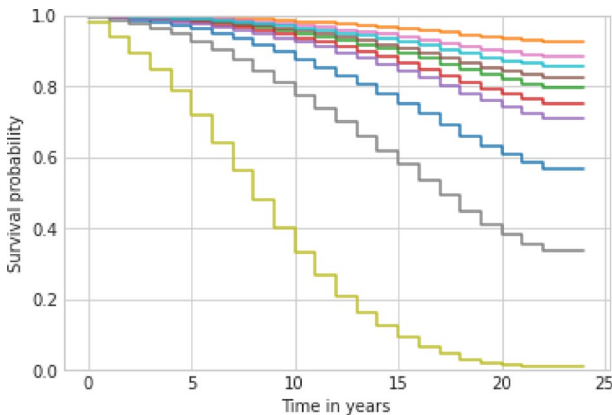
Fig. 22 10 policyholders’ survival curve for r^{acceptant} with GBSM
