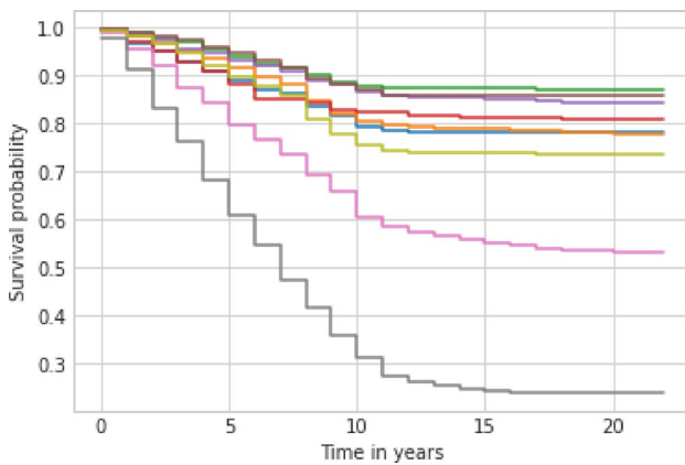
Fig. 21 10 policyholders' survival curve for r^{lapses} with RSF
