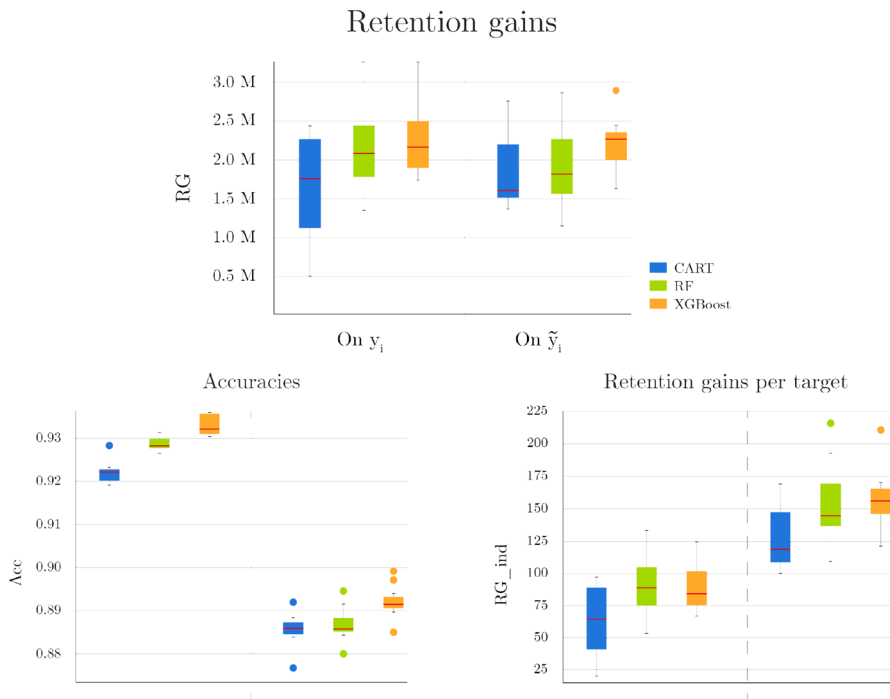
Fig. 6 Strategy no A-25: (Results on y_i better than results on \tilde{y}_i )
