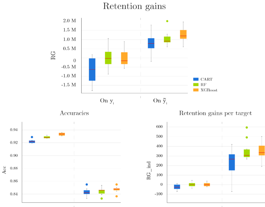
Fig. 4 Strategy no B-27: (Negative result on y_i and positive one on \tilde{y}_i )
