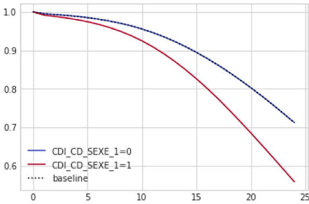
Fig. 17 r^{acceptant} trajectories by gender
