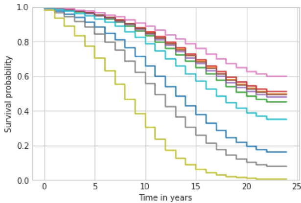
Fig. 23 10 policyholders' survival curve for r^{lapses} with GBSM
