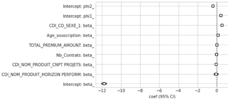
Fig. 16 Coefficient plot for r^{acceptant}
