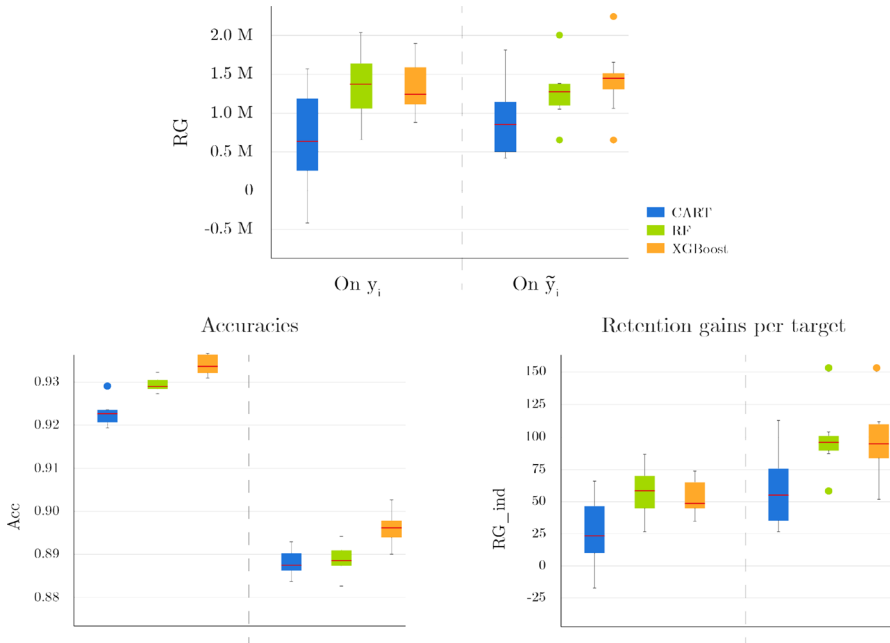
Fig. 5 Strategy no B-6: (High positive result on y_i slightly improved with \hat{y}_i )
