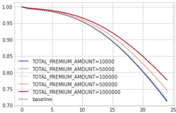
Fig. 19 r^{acceptant} trajectories for different face amounts
