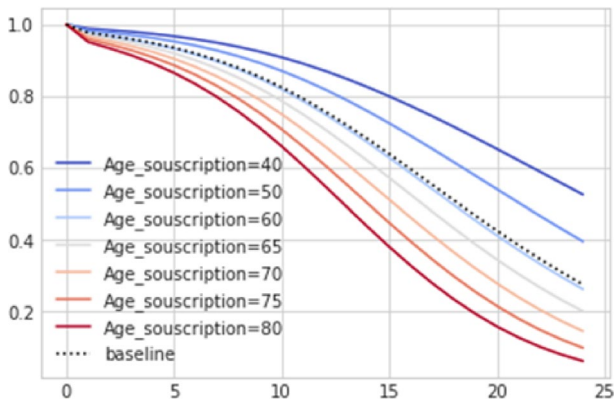
Fig. 14 p^{lapse} trajectories for different ages
