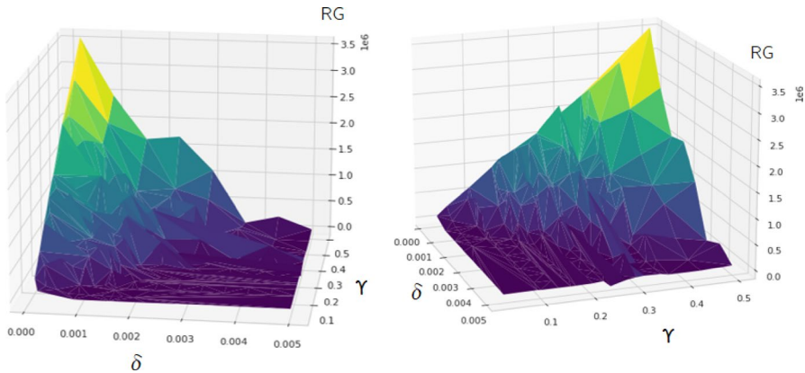
Fig. 7 3d plot (\delta, \gamma, RG)
