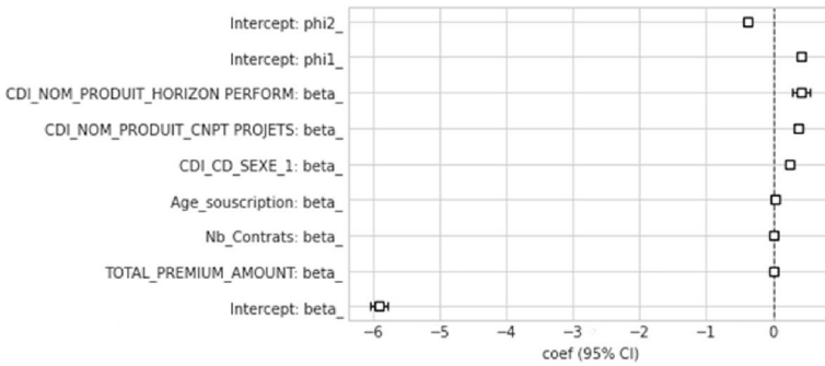
Fig. 11 Coefficient plot for r^{lapser}
