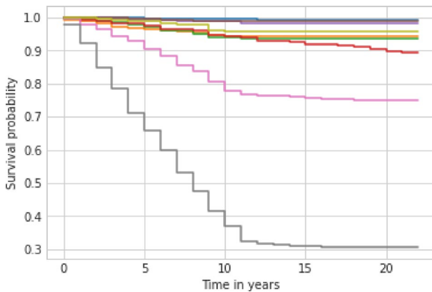
Fig. 20 10 policyholders' survival curve for r^{acceptant} with RSF
