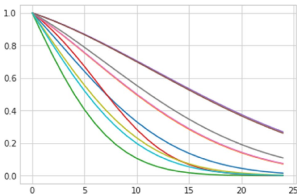
Fig. 10 10 policyholders' survival curve for r^{lapses}
