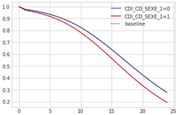
Fig. 13 p^{lapse} trajectories by gender
