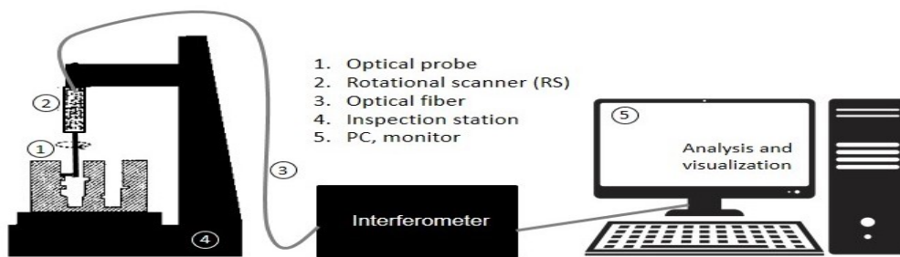
Figure 9: Optical bore-mapping system
