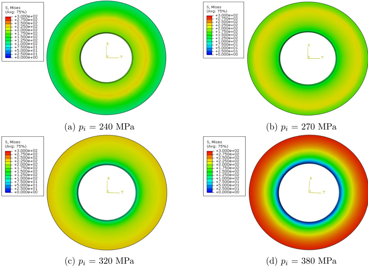
Figure 5: von-Mises stress distribution in gun barrel at various autofrettage pressure
