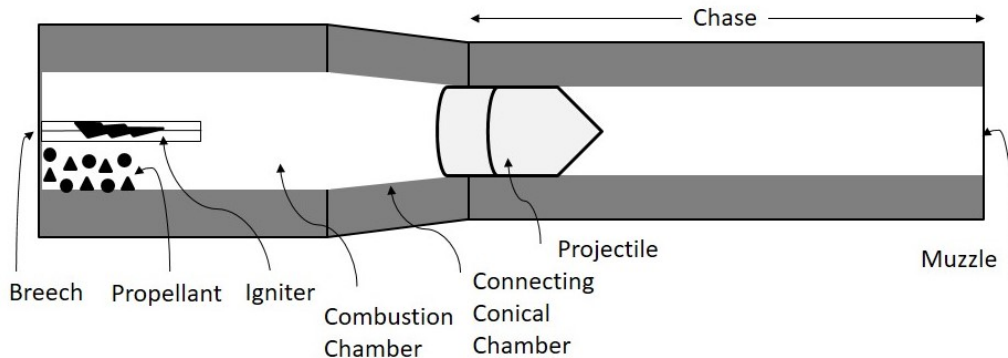
Figure 2: Firing of a projectile through barrel
