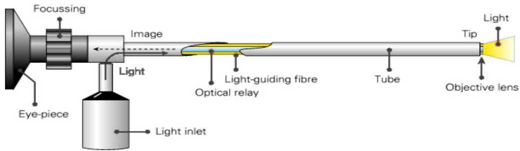
Figure 8: Side view of a rigid borescope (www.cryptomuseum.com)
