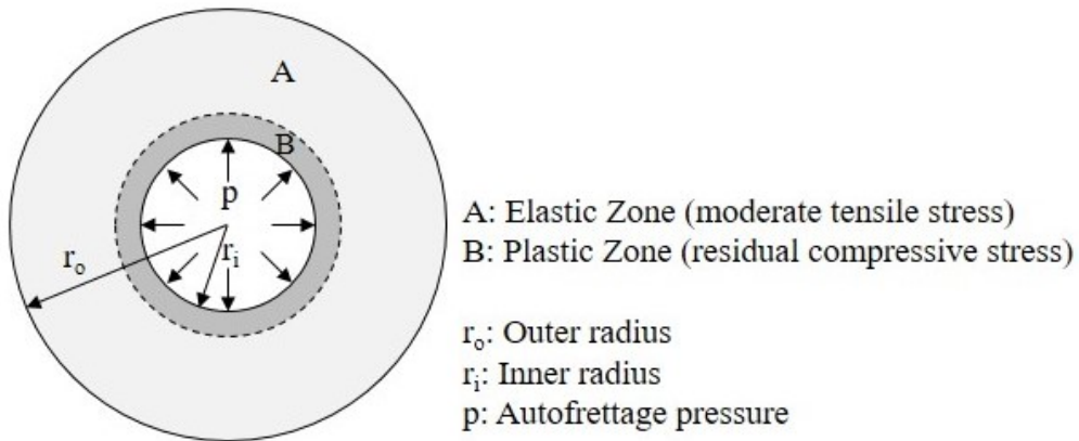
Figure 7: Creation of elastic-plastic region after autofrettage
