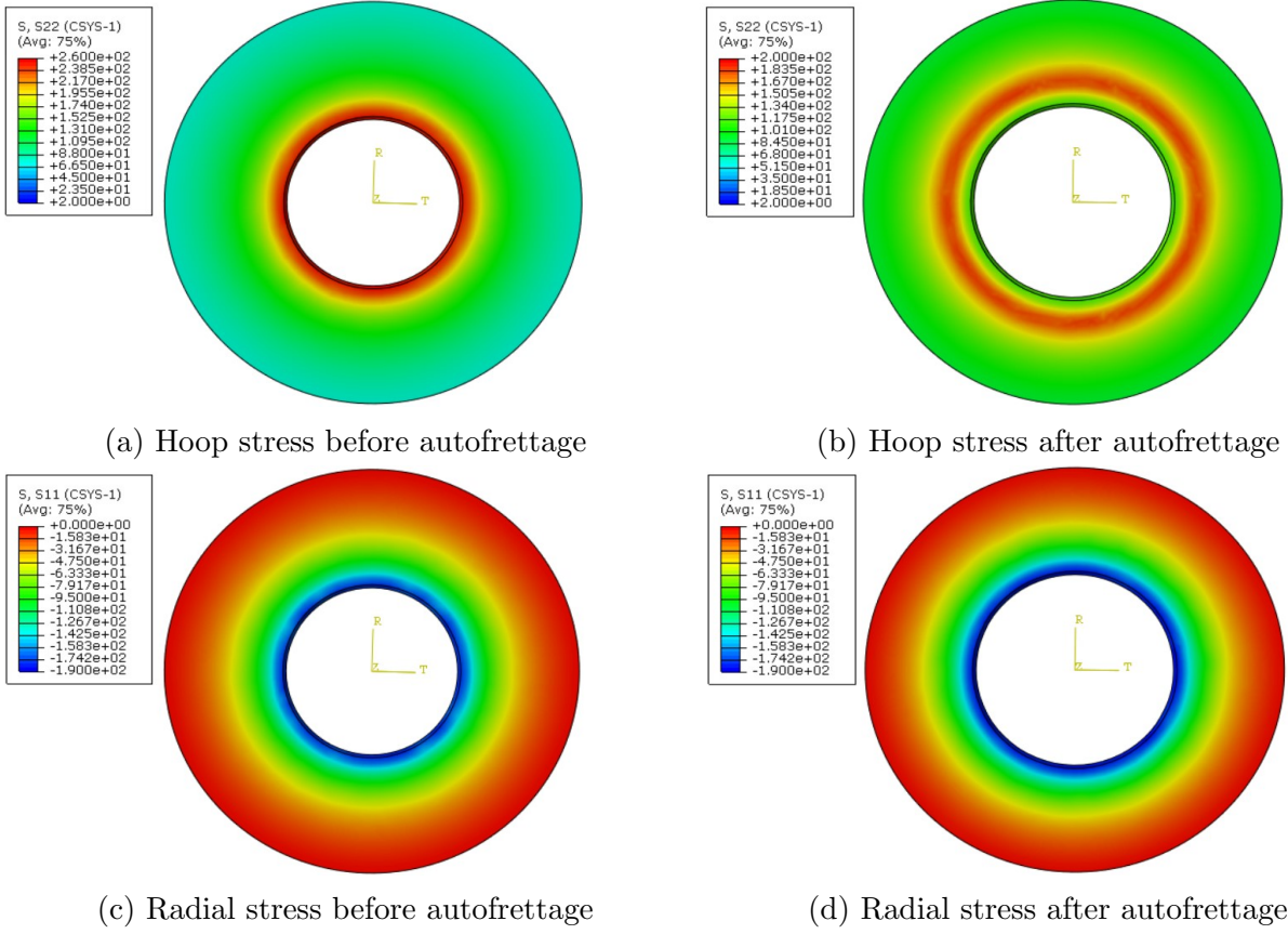
Figure 4: Stress distribution in a cylindrical gun tube before and after autofrettage
