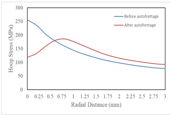
(a) Hoop stress before and after autofrettage
