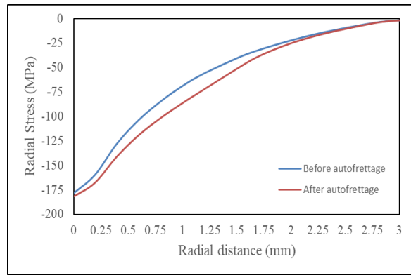
(b) Radial stress before and after autofrettage
