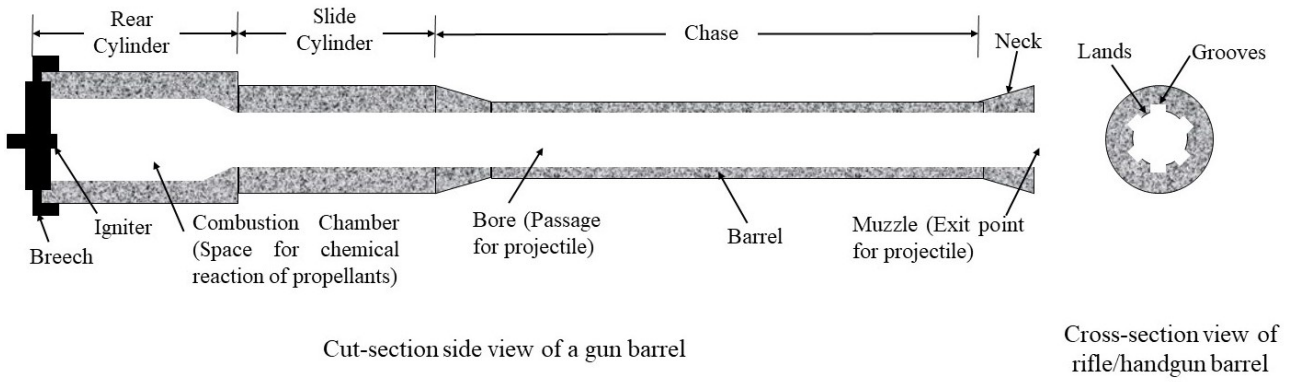
Figure 1: Typical design and components of a gun barrel
