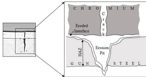
Figure 11: Magnified image of a microscopic crack due to thermochemical erosion
