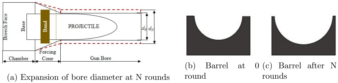
Figure 10: Schematic diagram of barrel failure mechanism due to the projectile's rotating band, (considering barrel is discarded after 'N' rounds)
