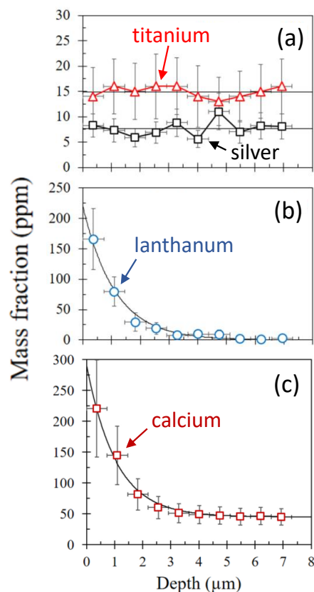
Figure 10: Trace element fractions of heavy flint glass (Schott, SF5) versus depth measured via depth-resolved calibration-free LIBS. (Adapted from Ref. [29])
