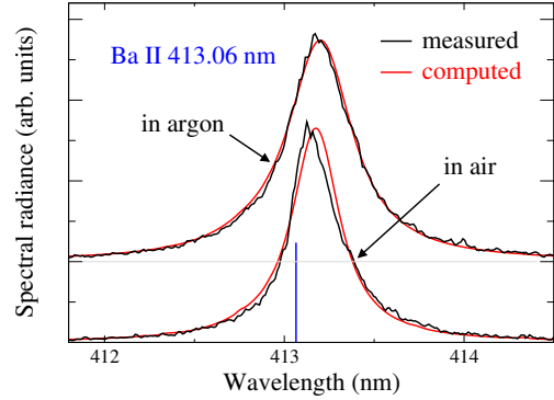
Figure 4: Ba II 413.06 nm line profile recorded during laser ablation of barite crown glass for t = 500 ns. Comparison to the spectral radiance computed for a uniform LTE plasma. The blue line indicates the resonance wavelength of the transition. (Adapted from Ref. [25])
