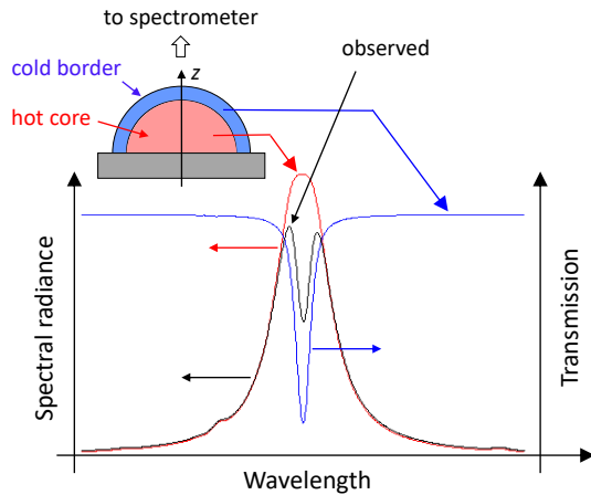
Figure 5: Illustration of the line shape of a strongly self-absorbed resonance line emitted from a nonuniform plasma. The large line profile emitted from the hot core is reabsorbed by the cold border in a narrow spectral range close to the resonance wavelength, according to the reduced electron density. The observed line shape exhibits thus an absorption dip.
