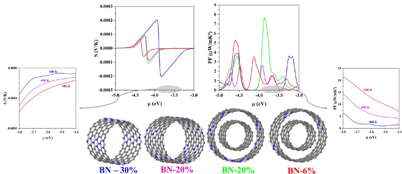
Figure 22. Transport properties of C@(BN)_x C_{1-x} zigzag double-walled nanotubes with different percentages and patterns of doping compared with the corresponding single-walled materials, (BN)_x C_{1-x} . Seebeck coefficient (left) and power factor (right). In the two insets: the dependency on temperature of S (left) and PF (right) in the range of chemical potentials corresponding to experimentally measured carrier densities.
