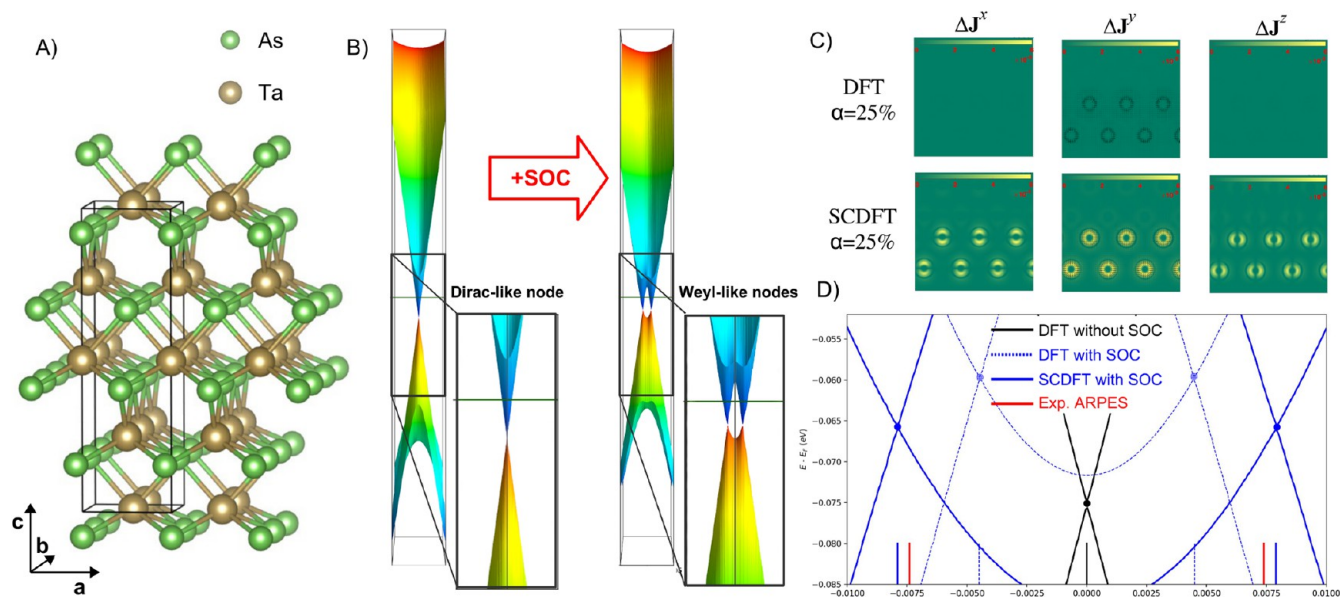
Figure 3. (A) Crystal structure of the I4_1md tetragonal phase of TaAs. (B) Effect of SOC on the valence band structure. (C) Orbital-relaxation contribution to the spin-current densities \Delta\mathbf{J}^i = \mathbf{J}_{\text{final}}^i - \mathbf{J}_{\text{initial}}^i with differences taken with respect to second variational values in the DFT (upper panels) and SCDFE (lower panels). (D) Splitting by SOC of the Dirac-like node into Weyl node pairs in the DFT and SCDFE and comparison with ARPES experimental values. 81
