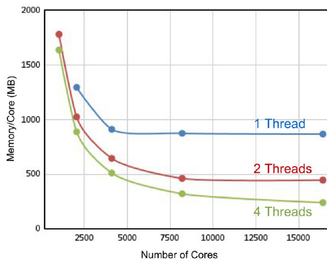
Figure 17. Memory usage per core of MPPCRYSTAL for the MCM-41 X16 case as a function of the number of cores and threads. All calculations were run on the Archer2 supercomputer.
