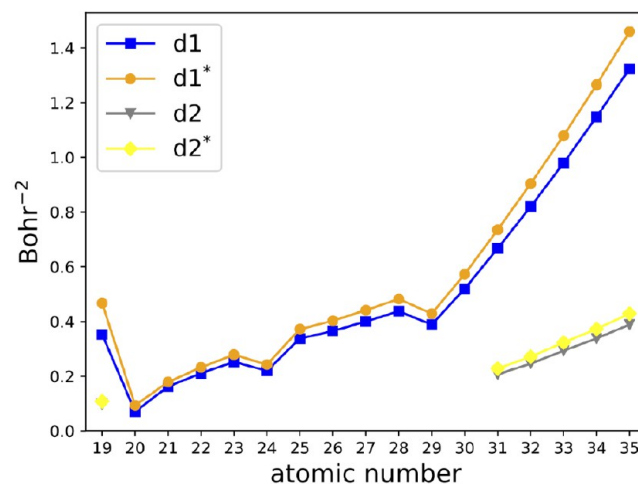
Figure 9. Example of revision of the def2-mSVP basis set: d exponents for the elements of the fourth row before (gray and blue lines) and after (yellow and orange lines) the basis set revision. d 1 is the exponent in the inner Gaussian function, while d 2 is the one of the outermost one.
