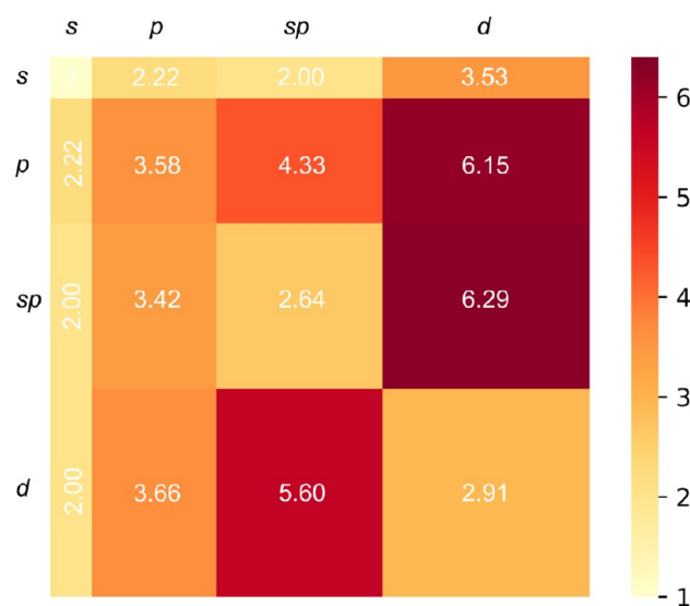
Figure 12. Speedups for calculating s - s , s - p , p - s , p - p , and d - d RSSH-GTF pair G_x^a , G_y^a , and G_z^a coefficients with the new routines in CRYSTAL23 vs the previously existing routines.
