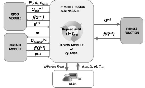
Figure 1: Simplified scheme of the unified algorithm.
