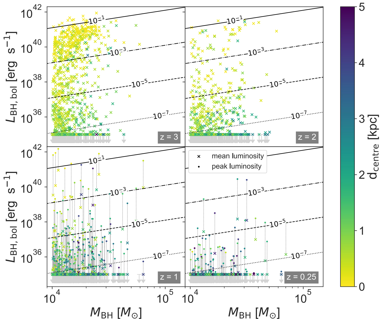
Figure 6. BH bolometric luminosity versus BH mass for all main BHs in dwarf galaxies, i.e. with stellar mass below M_{\text{dwarf}} = 3 \times 10^9 M_{\odot} . Points are coloured by the distance between the BH and the centre of the host galaxy. Mean luminosities over \pm \Delta t = 100 Myr are shown for all redshifts (crosses), with BHs with mean L_{\text{bol}} < 10^{35} \text{ erg s}^{-1} plotted at 10^{35} \text{ erg s}^{-1} as upper limits. For z \leq 1 , peak luminosities over the same \Delta t are also shown (dots). Constant Eddington fractions f_{\text{Edd}} are shown as black lines.
