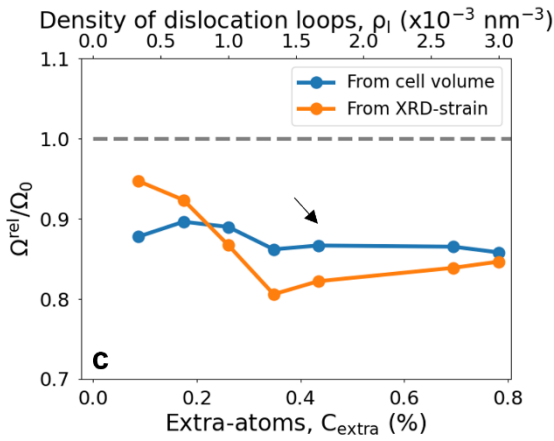
Fig. 7. Relaxation volume per extra-atom for a) one \langle 100 \rangle dislocation loop of varying radius, b) 20 \langle 100 \rangle loops of varying radius, c) varying number of \langle 100 \rangle loops of radius 6 u.c., as a function of extra-atom concentration ( C_{extra} ) and either radius ( R_l ) or density ( \rho_l ) of loops. \Omega^{rel} is given in atomic volume unit. Dashed line in inset in Fig. 7a shows \Omega^{rel} fitted with Eq. ( 6 ). Black arrows point to dots corresponding to two, independent cells with the same defect characteristics (20 \langle 100 \rangle dislocation loops of radius 6 u. c.)
