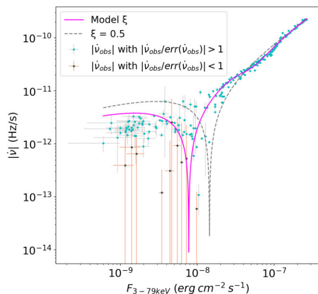
Figure 5. Plot of the absolute value of the frequency derivative |\dot{\nu}| versus the X-ray flux F_{3-79\text{keV}} for J0243. The symbols indicate the observational values from Fermi /GBM, the solid magenta line shows the prediction of our best-fitting model with \xi(\dot{m}) given by equation (13), and the dashed line shows the best-fitting model using the standard approach with a constant \xi = 0.5 .
