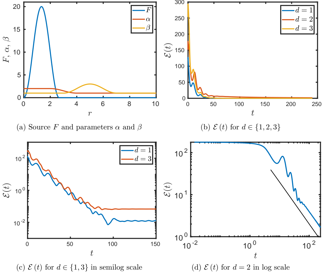
FIGURE 1. Large-time convergence for the radially symmetric example with the data as in (B.1)–(B.3).
