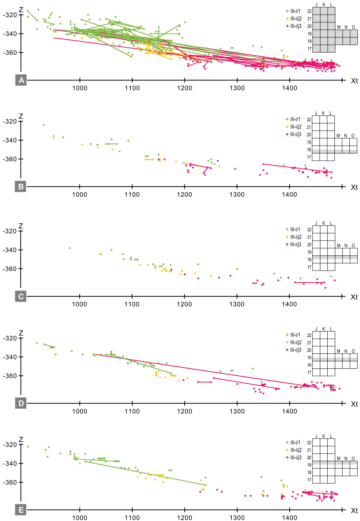
Fig. S12. Vertical distribution along the E-W axis of the grid of the lithic assemblages from layer III-i/j. A. Entire excavated area of the layer. B. North half of row 18 only. C. South half of row 18 only. D. North half of row 19 only. E. South half of row 19 only. The scatter graphs feature all piece-plotted lithics (for the purposes of these representations, the sieve items in refit units were also included; they were assigned the [x,z] coordinates of the center of the square meter or quarter-square meter of provenience, with elevation set at the mid-point of the stratigraphic unit's thickness).
