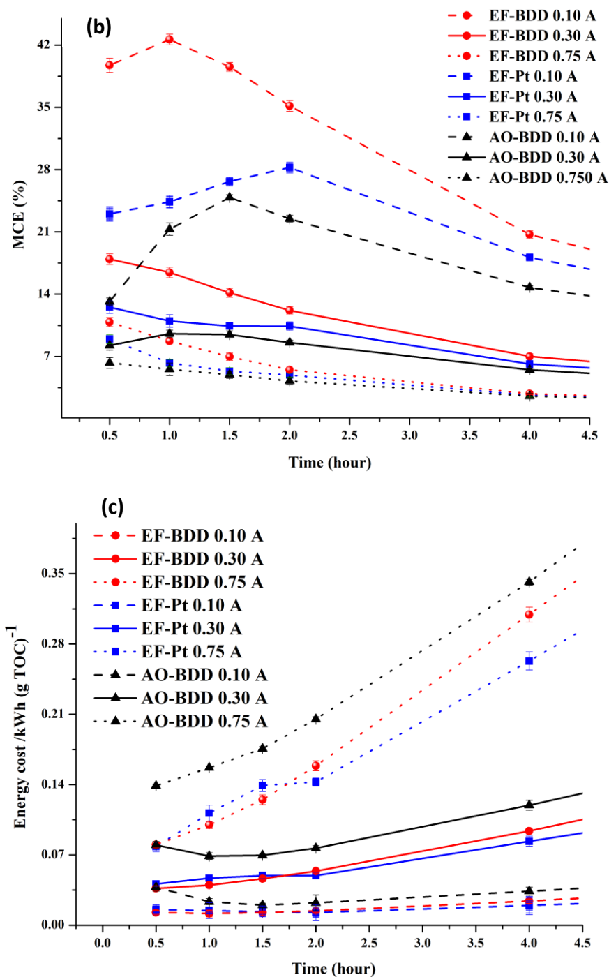
Fig. 3. (a): Linear relationship of -\ln(C_t/C_0) and operation time; (b): MCE value (%) of mineralization of NAX by \bullet\text{OH} and (c): Energy cost of mineralization of NAX under different current intensities in EAOPs. [\text{NAX}]_0 = 0.198 mM; [\text{Na}_2\text{SO}_4] = 50 mM; V = 0.25 L; for EF: [\text{Fe}^{2+}] = 0.10 mM; \text{pH} = 3.0 ; for AO: \text{pH} = 7.5 .
