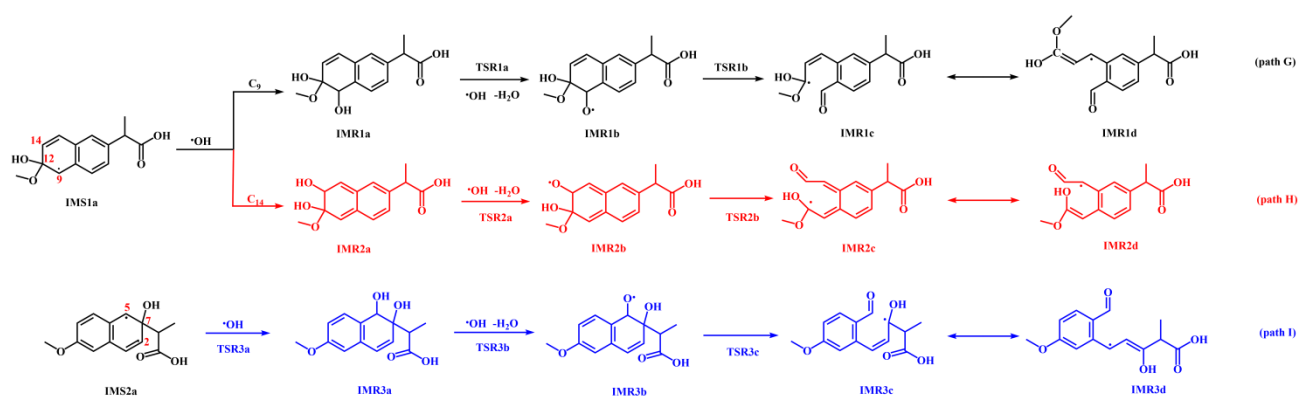
Fig. 7. “Ring-opening” reaction of \bullet\text{OH} and NAX at \text{C}_{17} and \text{C}_{18} with calculated intermediates (path G-I).
