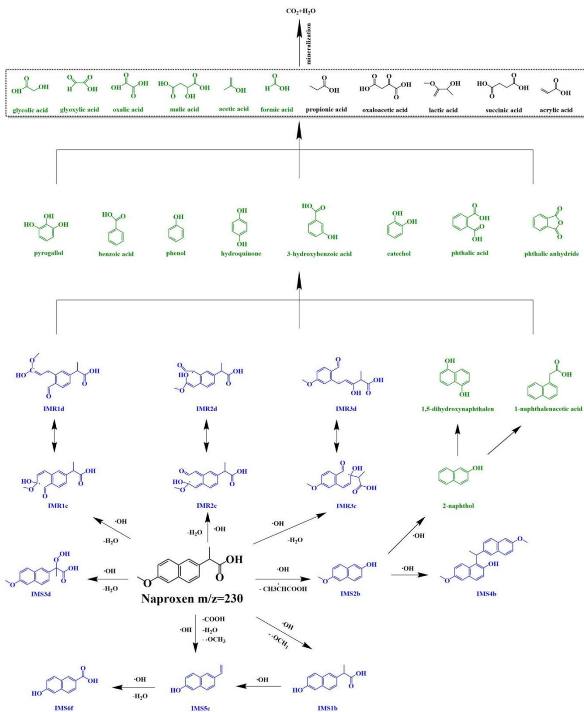
Fig. 8. General reaction pathway proposed for the mineralization of naproxen in aqueous medium by \bullet\text{OH} . Blue: DFT calculated; Green: detected in this research; Black: carboxylic acids validated by other research works.
