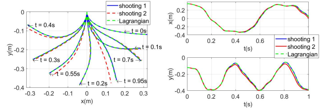
Fig. 4: Rod of test 1 with k = k_*/100 , pulled with an horizontal force and released from a highly deformed configuration: Snapshots (a), and time-evolution of the tip coordinates (b). The color code is the same as in figure 3.a.
