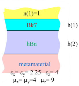
Fig. 10 Isotropic magnetic materials.
