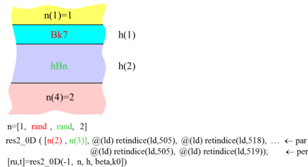
Fig. 9 Dispersion with anisotropy.
