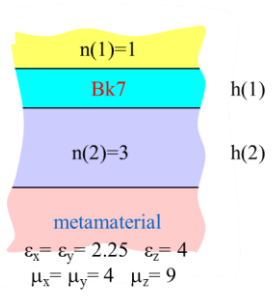
Fig. 11 Anisotropic magnetic materials.
