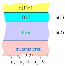
Fig. 10 Isotropic magnetic materials.
