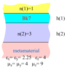
Fig. 11 Anisotropic magnetic materials.
