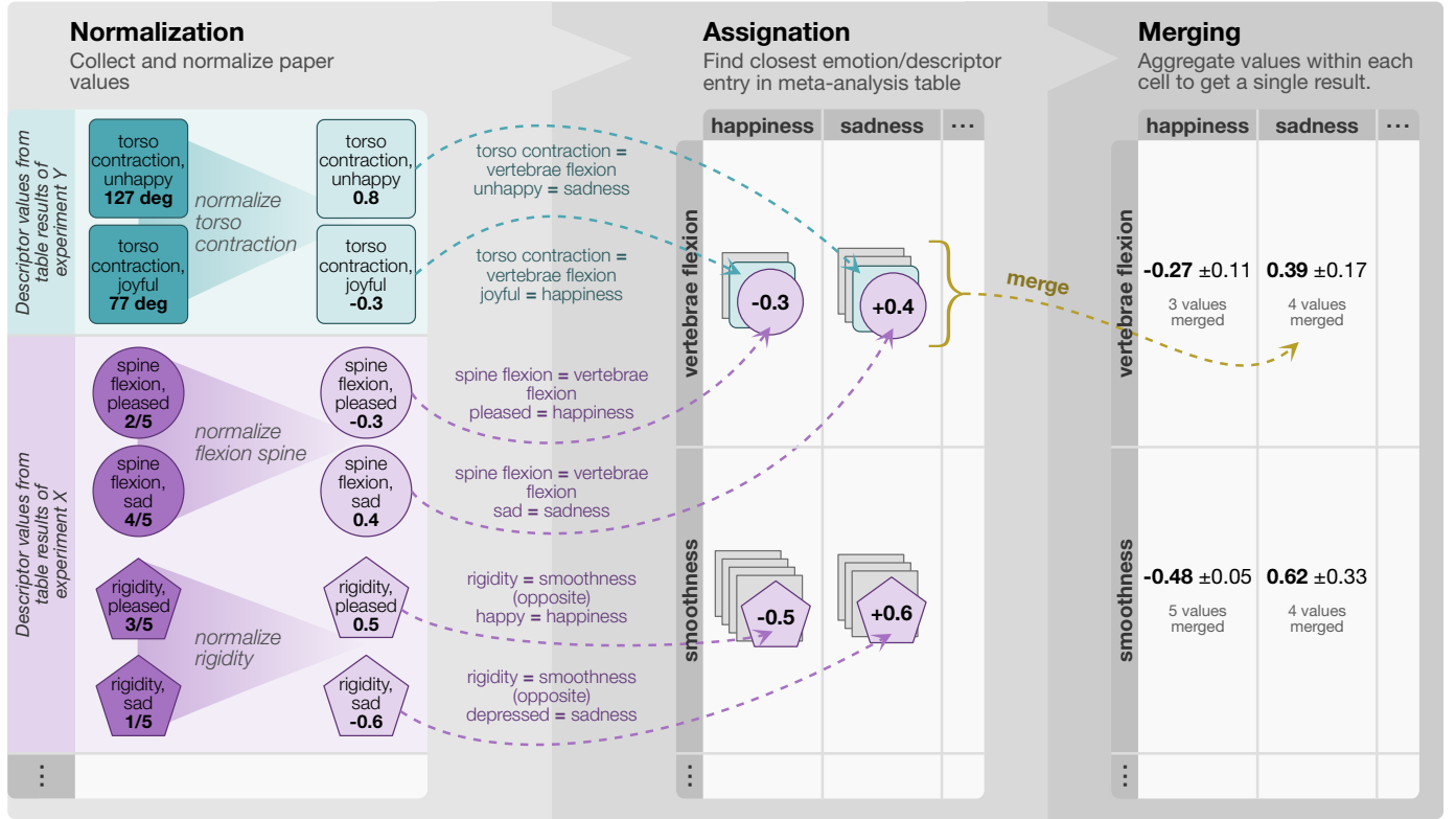
Fig. 1. Overview of the aggregation strategy employed for the meta-analysis and decomposed in three steps: normalization, assignment and merging. Numerical results above are only given as examples.
