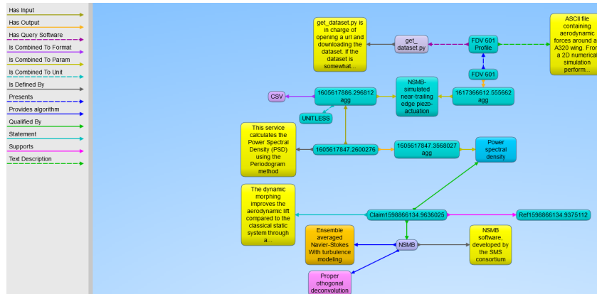
Figure 4: Elements of service composition in the ontology through browsing in Gruff, provided by Allegro
