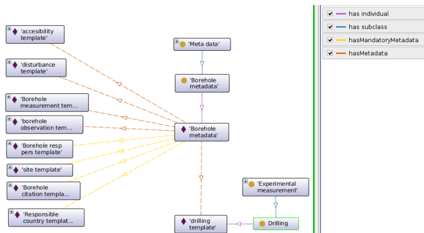
Figure 2: Modeling of Borehole metadata elements in HiperBorea instance of ARCAS
