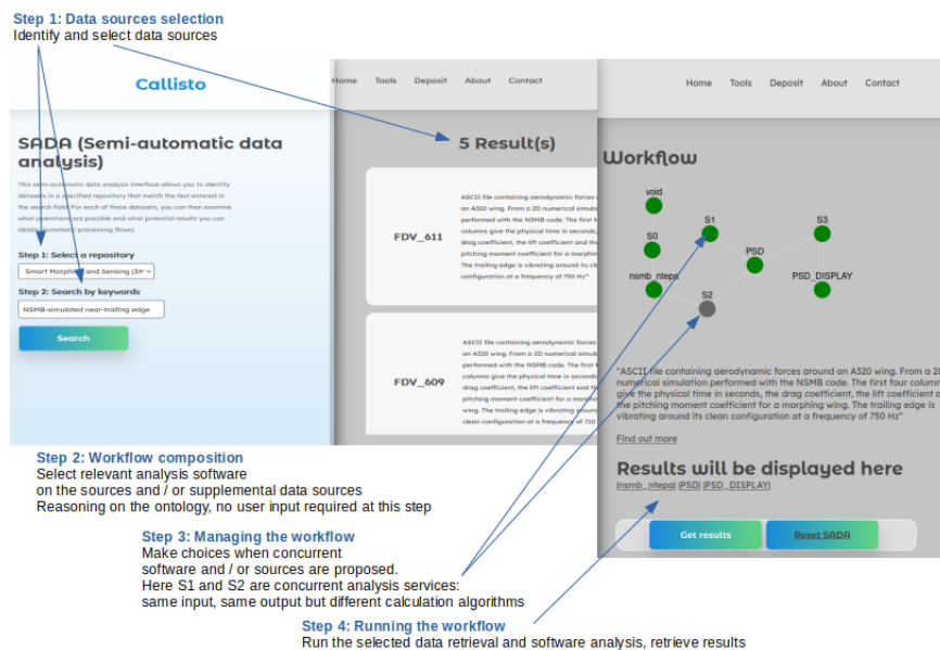
Figure 3: Service composition in CALLISTO
