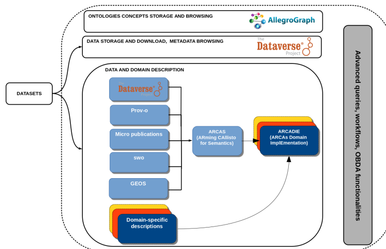
Figure 1: Functional overview of CALLISTO
