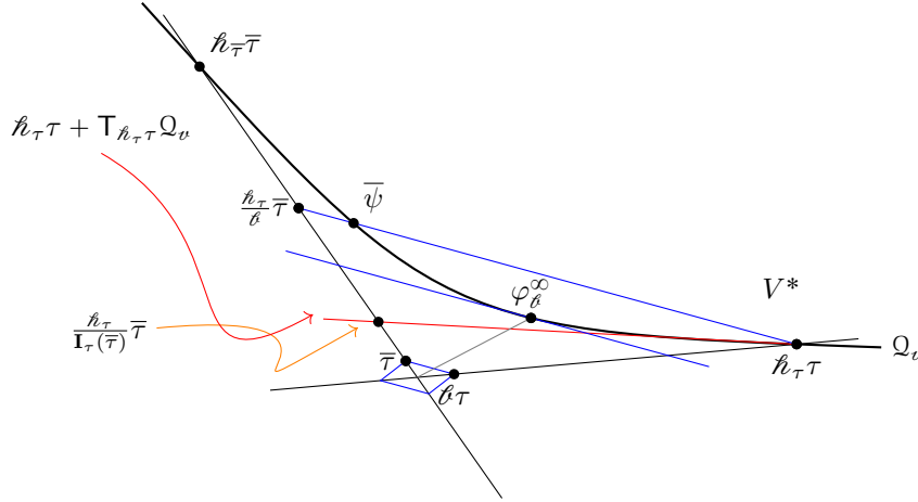
FIGURE 6. The situation of Lemma 5.9.
