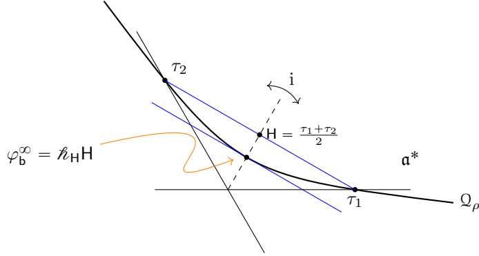
FIGURE 4. The critical hypersurface of a strictly convex projective structure on S . Since H is a convex combination of \{\tau_1, \tau_2\} one has \|H\|^1 = 1 and thus \|\varphi_b^\infty\|^1 = \ell^H .
