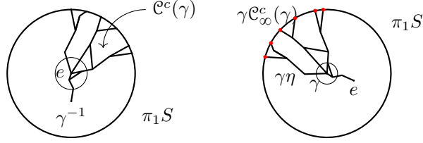
FIGURE 2. The coarse cone type of \gamma \in \Gamma (left). The set \gamma \cdot \mathcal{C}_\infty^c(\gamma) (right). Pictures from P.-S.-Wienhard [43].
