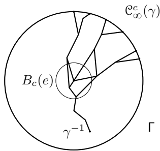
FIGURE 5. The coarse cone type at infinity, picture from P.-S.-Wienhard [42].
