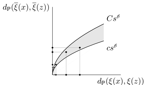
FIGURE 1. A \ell -concave point x . The marked points on the axis' represent d_{\mathbb{P}}(\xi(x), \xi(y_k)) and d_{\mathbb{P}}(\bar{\xi}(x), \bar{\xi}(y_k)) respectively.
