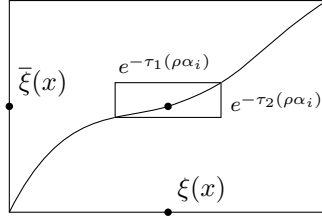
FIGURE 3. The image of the cone type \alpha_i \mathcal{C}_\infty^c(\alpha_i) by the graph curve \mathcal{E} in the C^{1+\nu} -torus \partial\Omega \times \partial\Omega^* .
