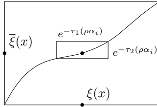
FIGURE 2. The image of the cone type \alpha_i \mathcal{C}_\infty(\alpha_i) by the graph curve \mathcal{G} in the \mathbb{C}^{1+\text{H\"ol}} -torus \partial\Omega \times \partial\Omega^* .
