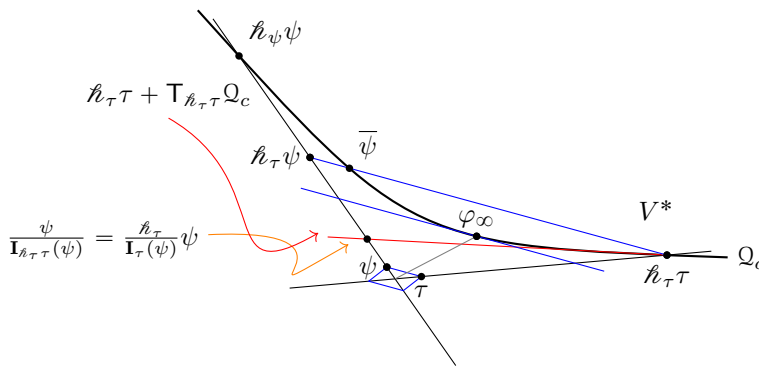
FIGURE 4. The situation of Lemma 3.6.
