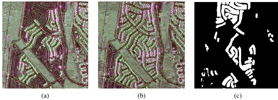
Fig. 5. UAVSAR images (in Pauli decomposition) on April 23, 2009 and May 11, 2015. (a) before change. (b) after change. (c) ground truth where white color is change and black color is no-change.
