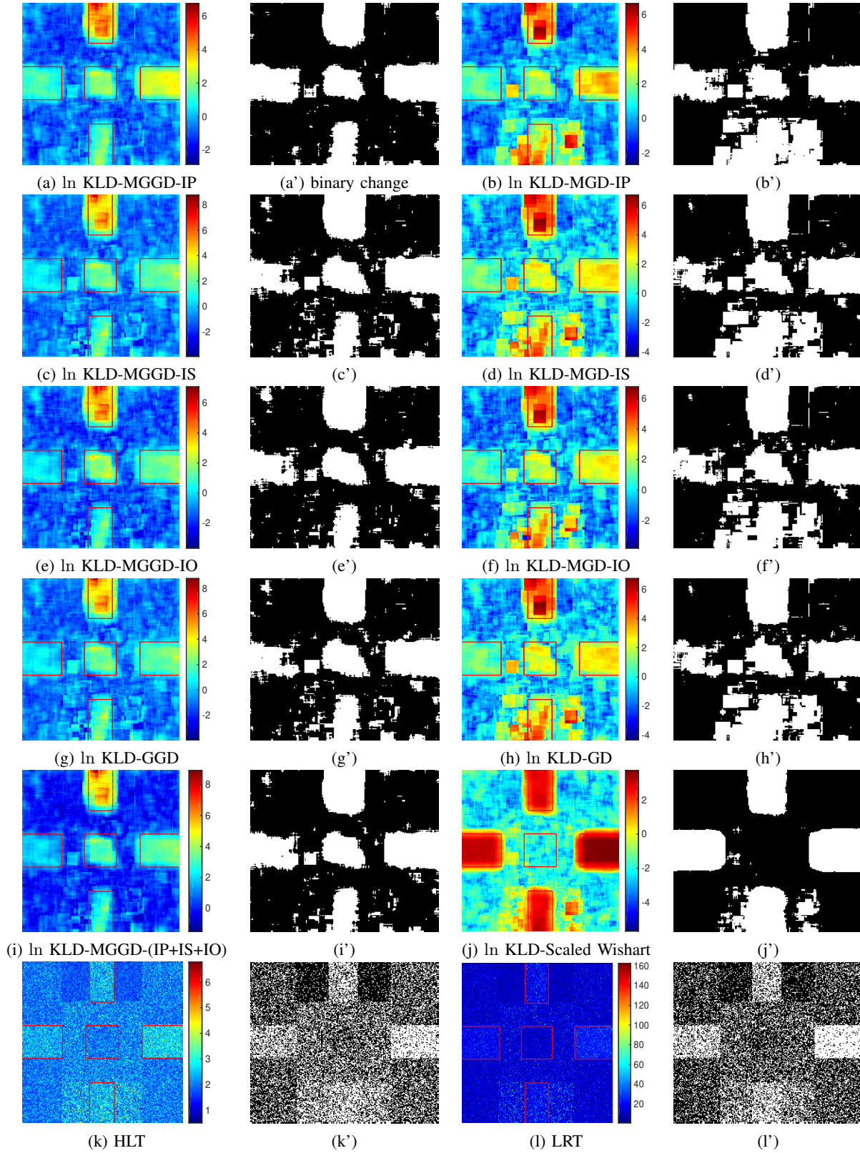
Fig. 3. Detection results for simulated PoSAR data. (a) and (b) \ln KLD for IP dependence with MGGD and MGD, and their corresponding binary change maps (a')-(b') where white color is change and black color is no-change. (c)-(d) \ln KLD for IS dependence with MGGD and MGD, and their binary maps (c')-(d'). (e)-(f) \ln KLD IO dependence with MGGD and MGD, and (e')-(f') their binary maps. (g)-(h) \ln KLD for univariate GGD and GD, and their binary change maps (g')-(h'). (i) and (i') \ln KLD-MGGD (IP+IS+IO) dependence with MGGD and binary map. (j) and (j') \ln KLD with scaled Wishart and corresponding binary map. (k)-(l) results of the HLT and LRT methods. Parameters used: sliding window size = 16, wavelet transform scale L = 1 , Daubechies wavelet filter: db1. Optimal threshold selected corresponds to the closest point to (0.0, 1.0) in the ROC curve.
