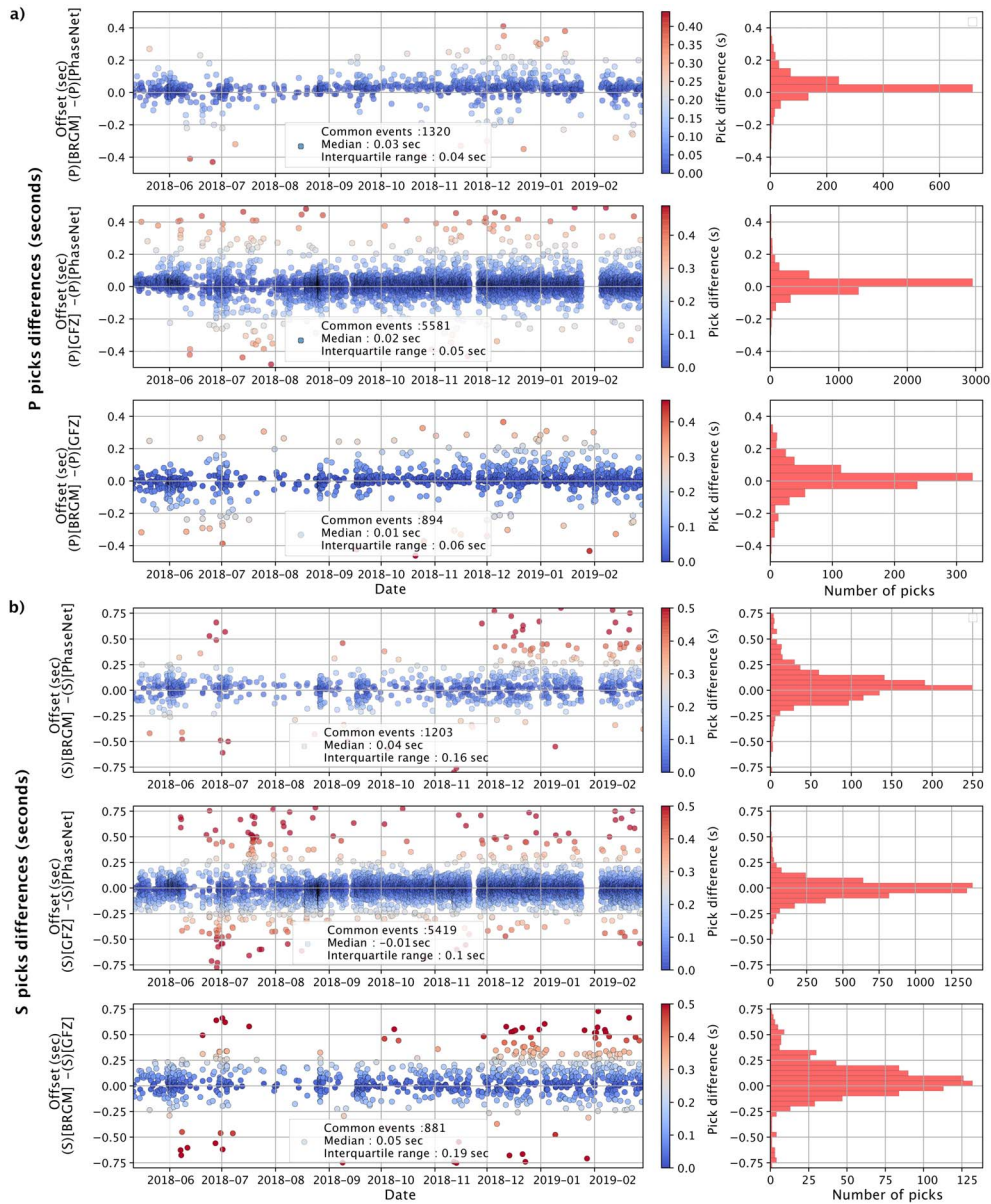
Figure 2. (a) P-pick time differences (left, for each event; right, distribution for all events). From top to bottom: comparison between PhaseNet and BRGM catalogues, comparison between PhaseNet and GFZ catalogues, comparison between GFZ and BRGM catalogues. Outliers are not represented. (b) Same as (a) for S-picks.
