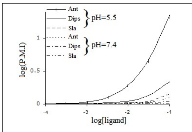
Fig. 4: Mobilization of copper(II) in simulated extracellular fluid in the presence of Dips, Ant and Sla at physiological (7.4) and inflammatory (5.5) pH values.
