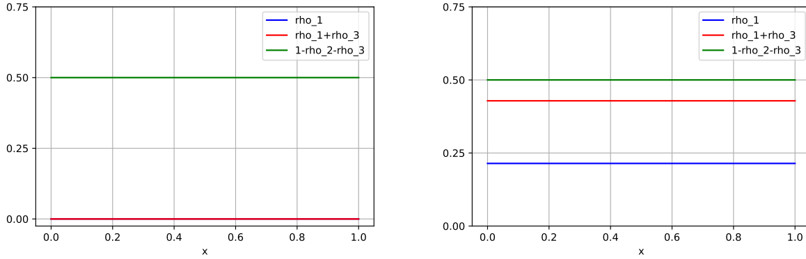
(a) (\rho_1, \rho_1 + \rho_3, 1 - \rho_2 - \rho_3)(T, \cdot) , solution of (B.1) with initial condition (0, 0, 0) .
