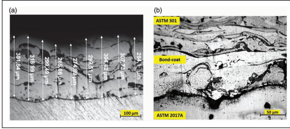
Figure 2. Metallographic images of a wire arc sprayed stainless steel (ASTM 301) on aluminium substrate (ASTM 2017A). (a) Example of a 300 μm coating thickness. (b) Illustration of the layered structure of the coating.
