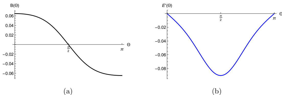
FIG. 9: (a) The magnetic and (b) the effective electric field, B = B(\vartheta) and \mathbf{E}^* = \nabla B , respectively, on the horizon of a Kerr-Newman black hole.
