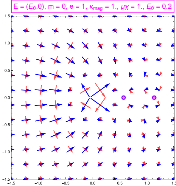
FIG. 7: Combining a constant external electric field \mathbf{E} = \mathbf{E}_0 with \nabla B induced by the spin-field term (II.21) yields effective electric field \mathbf{E}^* (IV.41). Velocity and force are perpendicular, as required by the Hall law. The number of equilibrium points has been considerably reduced.
