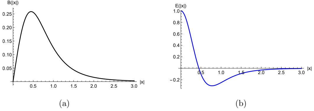
FIG. 4: (a) The planar magnetic field B(|\mathbf{x}|) in (IV.47) (b) induces a radial effective electric field \mathbf{E}^* = \nabla B .
