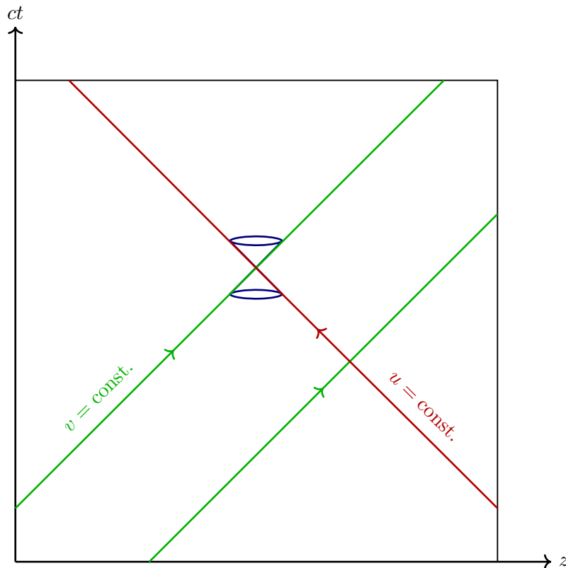
FIG. 2: Spacetime diagram. The light-cone is in blue . Photon trajectories are either outgoing ( \dot{z} > 0 ) depicted in green or ingoing depicted in red .
