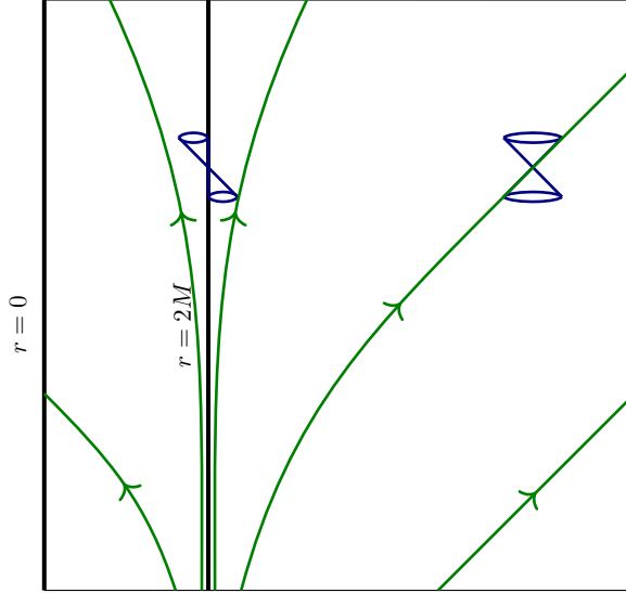
FIG. 8: Eddington-Finkelstein diagram of a Schwarzschild spacetime, with outgoing light rays u = \text{const.} in green, highlighting key features such as the singularity, the horizon, and different trajectories of outgoing photons. Infinitely far away from the black hole, space is Minkowskian. However, the closer we get, the more the gravitational field bends the light cones inward, resulting in outgoing photons taking an ever longer time to escape from the black hole region. Past the horizon, the light cone is completely bent inward such that the only future-pointing directions are toward the singularity. An outgoing photon emitted right on the horizon would have a vertical trajectory, thus staying on the horizon.
