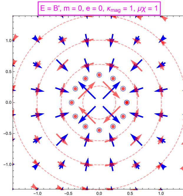
FIG. 5: For uncharged particles the radial planar magnetic field B in (IV.47) induces a radial effective electric field \mathbf{E}^* . An “exotic photon” i.e. a mass and chargeless planar Carroll anyon with nonzero spin \chi , magnetic moment \mu and magnetic charge \kappa_{\text{mag}} , (IV.45), rotates around the origin along concentric circles, consistently with the generalized Hall Law, (IV.42). The rotation stops on a ring of a fixed radius (marked by full dots in red ) where the effective electric field vanishes, \mathbf{E}^* = 0 , and its direction is reversed when \mathbf{E}^* changes sign.
