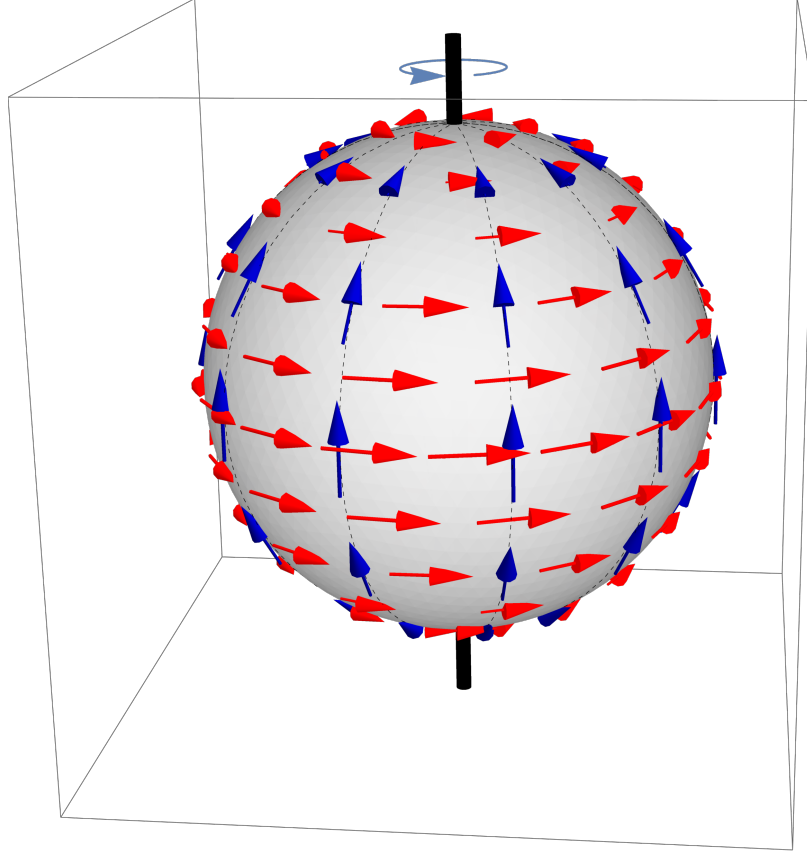
FIG. 10: The horizon of a Kerr-Newman black hole (topologically a two-sphere) rotates around its vertical axis. For an uncharged particle the usual EM fields are switched off but the spin-field term induces an effective electric field \mathbf{E}^* \propto \nabla B indicated by vertical blue arrows . The horizontal red arrows depict the velocity , (VI.18), of a massless, uncharged doubly-extended anyon on the horizon. The force and the velocity follow the Hall law (I.2) which, in the case of the Kerr-Newman black hole, has the form of (VI.18).
