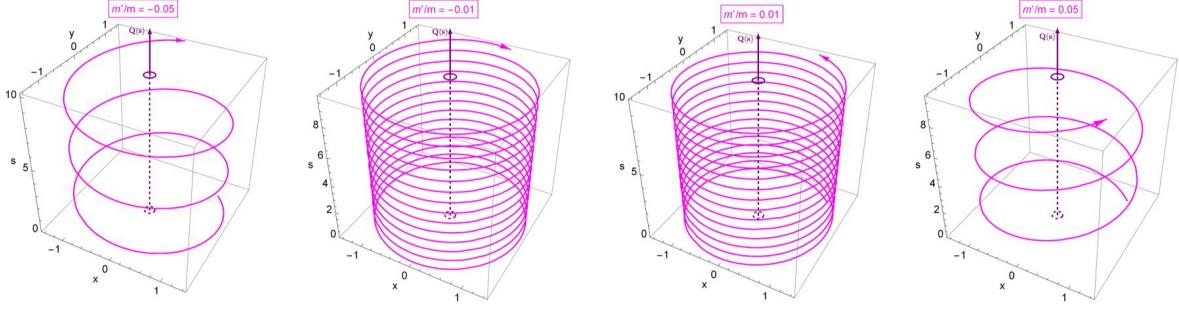
FIG. 3: Trajectories for unit charge and exotic parameter in a radial electric field \mathbf{E} = \mathbf{x}/|\mathbf{x}|^3 in the plane for effective masses passing from negative to positive, unfolded in Carroll time s . The rotation around the fixed guiding center \mathbf{Q}(s) = \mathbf{Q}_0 speeds up when the effective mass increases from m^* < 0 . The motion is instantaneous for m^* = 0 and changes orientation for m^* > 0 .
