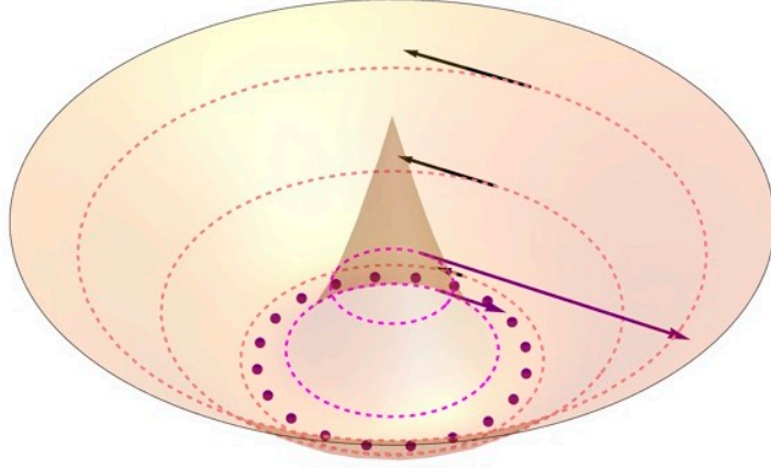
FIG. 6: The motion of an anyon in the effective electric field \mathbf{E}^* can be lifted to “Mexican Hat” potential surface -B(|\mathbf{x}|) above the plane. The trajectories are horizontal “cords” (circles) starting near the “top” with high velocities and, then decreasing progressively until we arrive at |\mathbf{x}| = |\mathbf{x}_0| where the force vanishes, \mathbf{E}^*(|\mathbf{x}_0|) = 0 , and the rotation stops. The “cord” degenerates to fixed points around the “bottom rim”. Then, as we climb up the outer “flange” by letting |\mathbf{x}| increase, the anyon restarts to move with ever increasing velocity — however in the opposite direction. The 3D picture projects to Fig. 5.
