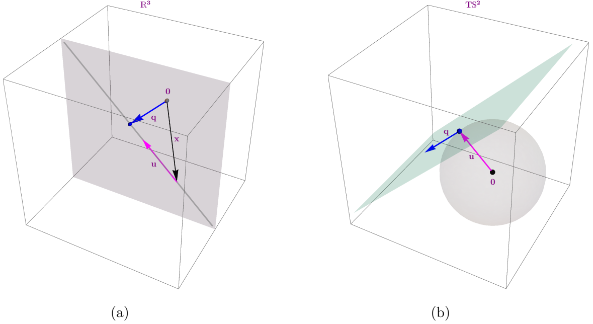
FIG. 1: (a) A Fermat particle in flat space moves along oriented straight lines. The unit vector \mathbf{u} gives its direction and the vector \mathbf{q} points to its closest point to a (chosen) origin. \mathbf{x} is any point on the ray. (b) The space of motions is thus the tangent bundle of the unit 2-sphere, endowed with k -times its canonical symplectic form.
