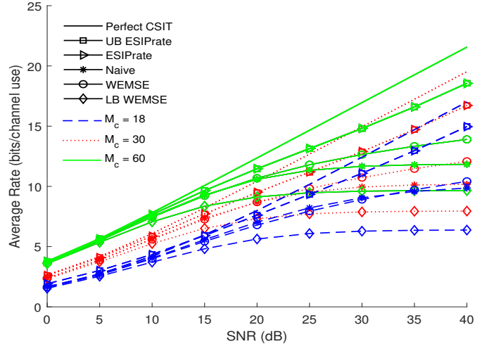
Fig. 1: Average Rate with Partial CSIT vs. SNR, C = 2, K = 3, \rho_D = 10, N_r = d_k = 2 .
