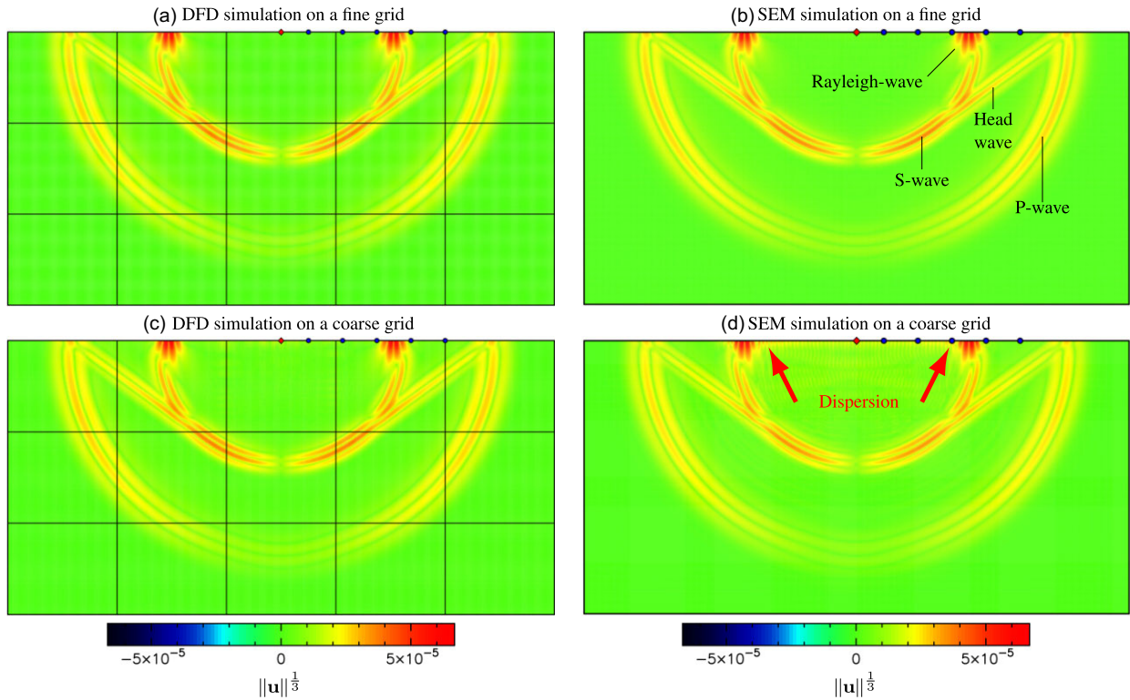
Figure 7. The snapshots show the magnitude of the displacement vector for four different simulations at time t = 0.85 s. The magnitude of the displacement is raised to the power 1/3 to enhance waves having a small amplitude. The velocity model has dimensions 6400 m by 3200 m with P -wave velocity v_p = 3400 m s ^{-1} , S -wave velocity v_s = 1963 m s ^{-1} and density \rho = 2500 kg m ^{-3} . The waves are generated by an explosive source placed at the position marked by a red diamond. The source time function is a Ricker wavelet with peak frequency f_0 = 10 Hz. The receivers are represented using blue circles. The seismograms recorded in the simulations (a, b) and (c, d) are plotted in Figs 8 and 9, respectively. The different seismic waves are indicated in panel (b). Panel (a) shows the wavefield obtained for a DFD simulation with 15 domains. The grid has 168 780 gridpoints. The wavefield is represented with the fourth-order polynomial basis in Fig. 1(a). There are 12.2 points per P -wavelength and 7 points per S -wavelength. The time step is \Delta_t = 8.5 \times 10^{-4} . Panel (b) is similar to (a) but for a SEM simulation with 10 368 elements and 166 753 gridpoints. The number of points per wavelength and the time step are the same in panels (a) and (b). Panel (c) is similar to panel (a) but the grid is coarser. The grid has 42 630 points. The wavefield is represented using the fourth-order B-spline basis in Fig. 1(c); There are 6.1 points per P -wavelength and 3.5 points per S -wavelength. The time step is \Delta_t = 1.7 \times 10^{-3} . Panel (d) is similar to panel (c) but for a SEM simulation with 2592 elements and 41 905 gridpoints. The number of points per wavelength and the time step are the same in panels (d) and (c). In panels (a) and (b), there are enough points per wavelength. The P wave and the S wave are modelled accurately. There is no visible numerical dispersion, and the wavefields obtained using DFD and SEM are identical. In panels (c) and (d), the number of points per wavelength and the time step are divided by two with respect to panels (a) and (b). In panel (d), we see that the SEM simulation exhibits significant numerical dispersion for the surface wave, as indicated by the red arrows. In panel (c), we observe no numerical dispersion with the DFD, and the wavefield looks identical to panel (a).
