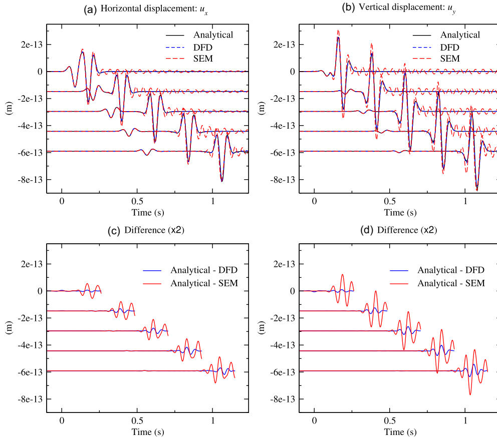
Figure 9. Comparison between the seismograms obtained using the DFD, SEM and the analytical solution when modelling surface wave propagation on a coarse grid, as detailed in Figs 7(b) and (c). Panels (a) and (b) show the horizontal and the vertical displacements, respectively. The recordings correspond to the five receivers represented by blue circles in Fig. 7. The seismograms obtained using the DFD (dashed blue lines) match perfectly the analytical solution (solid black line). The seismograms obtained using the SEM (dashed red lines) exhibit some spurious ringing in the surface waves because the number of points per wavelength is insufficient. Panels (c) and (d) show the difference (multiplied by 2) between the computed seismograms and the analytical solution. The difference in panels (c) and (d) are cut when the analytical solution predicts no more waves. The maximum difference between the analytical solution and the computed seismograms is about 8 and 25 per cent of the signals' amplitude for the DFD and SEM seismograms, respectively.
