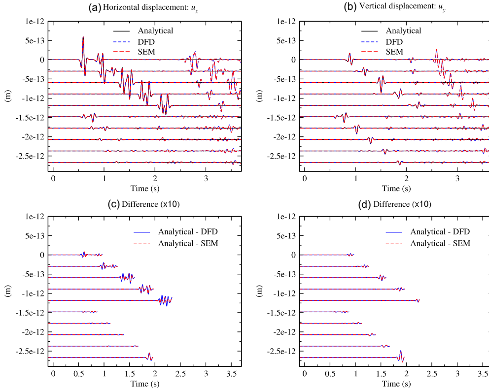
Figure 11. Comparison between the seismograms obtained using DFD, SEM and the analytical solution when modelling wave propagation near a solid–fluid interface on a fine grid, as detailed in Figs 10(a) and (b). Panels (a) and (b) show the horizontal and the vertical displacements, respectively. The recordings correspond to the ten receivers represented by blue circles in Fig. 10. The first five receivers are placed in the acoustic region, and the last five receivers are placed in the elastic region. Panels (c) and (d) show the difference (multiplied by 10) between the computed seismograms and the analytical solution. The differences in panels (c) and (d) are cut when the analytical solution predicts no more waves. The arrivals observed later in the computed seismograms come from reflections on the free surfaces at the sides of the domain. The maximum difference between the analytical solution and the computed seismograms is about 5 per cent of the signals’ amplitude in both simulations.
