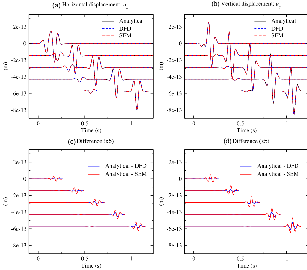
Figure 8. Comparison between the seismograms obtained using DFD, SEM and the analytical solution when modelling surface wave propagation on a fine grid, as detailed in Figs 7(a) and (b). Panels (a) and (b) show the horizontal and the vertical displacements, respectively. The recordings correspond to the five receivers represented by blue circles in Fig. 7. Panels (c) and (d) show the difference (multiplied by 5) between the computed seismograms and the analytical solution. The differences in panels (c) and (d) are cut when the analytical solution predicts no more waves. As expected, the numerical error increases with the distance to the source because of the accumulation of the numerical dispersion. The maximum difference between the analytical solution and the computed seismograms is about 2.5 and 5 per cent of the signals' amplitude for the DFD and SEM seismograms, respectively.
