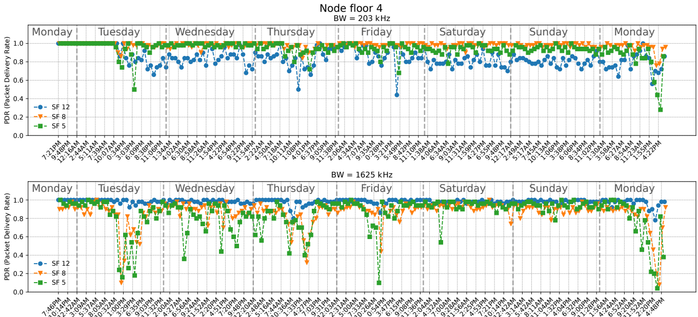
Fig. 7: Evolution of the PDR as a function of time, for six configurations (two BWs and three SFs), for the end node situated on the same floor as the gateway.
