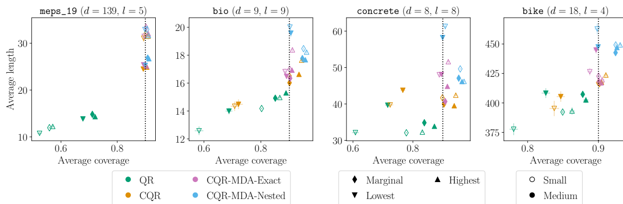
Figure 13: Model is NN. The mask is concatenated in the features. Data is imputed using Iterative Ridge. 100 repetitions are performed, allowing to display the standard error as error bars. The vertical dotted lines represent the target coverage of 90%.
