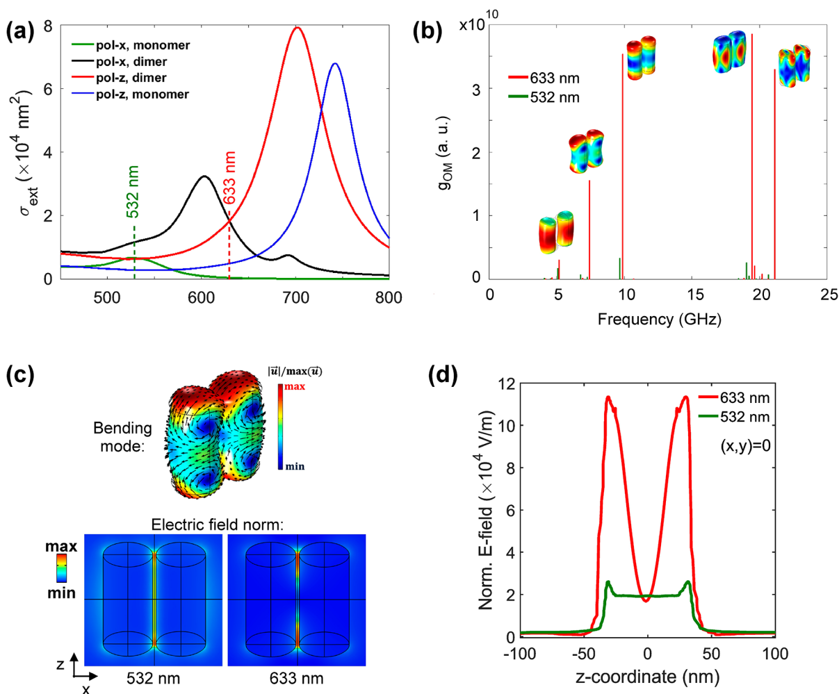
Figure 5. Plasmonic coupling and optomechanical calculations of the Au700 dimer in PVA. (a) The extinction cross-section as a function of wavelength for the Au700 monomer with x -polarization (green) and z -polarization (blue) and the Au700 dimer with polarization along the x -axis (black) and the z -axis (red). All these calculations employ the ellipsoid-capped NR geometry of the optomechanical model. The vertical dashed lines denote the wavelength of the laser excitation. (b) The optomechanical spectrum up to 25 GHz for the Au700 dimer averaged over the x - and z -polarizations. (c) The displacement field of the dimer bending mode (top) and the plasmonic near-fields for the two laser wavelengths (bottom) with x -polarized incident light. (d) The norm of the electric field along the z -coordinate, with (x, y) = 0 for the two laser wavelengths with x -polarized incident light.
