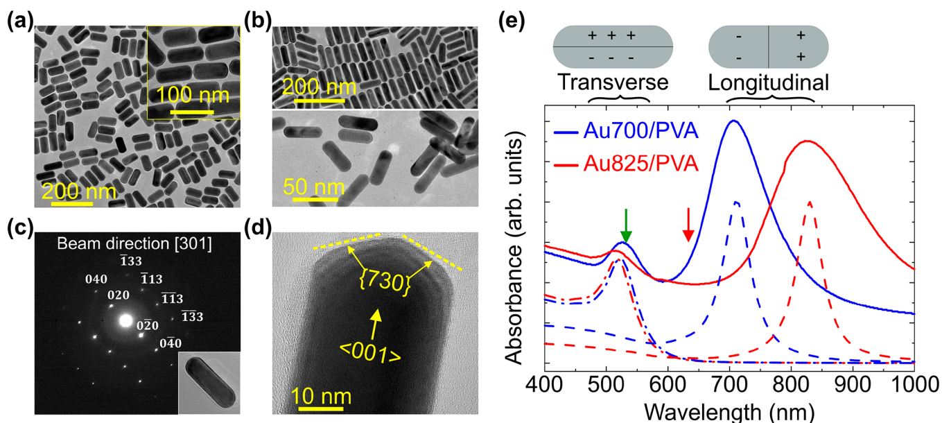
Figure 1. Structure and extinction spectrum of Au NRs. (a) TEM image of Au700 NRs and a higher magnification image shown as inset. (b) TEM images of Au825 (up) and Au800 (down) drop casted from a water suspension on standard TEM grids. (c) TEM diffraction pattern of a Au825 NR (inset) verifying its single-crystalline structure. (d) HR-TEM image and illustration of the \langle 001 \rangle crystal growth direction and the \{730\} surface facets of a single Au700 NR. (e) Experimental extinction spectra (solid lines) of Au700 (blue) and Au825 (red) dispersed in polyvinyl alcohol (PVA), and FEM calculations of the extinction cross-section of transverse (dashed dot) and longitudinal (dashed) single NR plasmons. For the calculated spectra, the terms “longitudinal” or “transverse” refer to the polarization of the incident light being parallel or normal to the \langle 001 \rangle axis of the Au NRs, respectively. The intensities of all curves have been scaled for comparison. The arrows correspond to the 532 nm (green) and 633 nm (red) laser wavelengths used for the BLS measurements.
