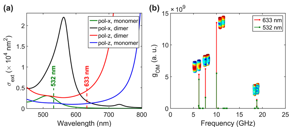
Figure 6. Plasmonic coupling and optomechanical calculations of the Au825 dimer in PVA. (a) The extinction cross section as a function of wavelength for the Au825 monomer with x -polarization (green) and z -polarization (blue), and the Au825 dimer with polarization along the x -axis (black) and the z -axis (red). (b) The optomechanical spectrum up to 25 GHz for the Au825 dimer averaged over the x - and z -polarizations.
