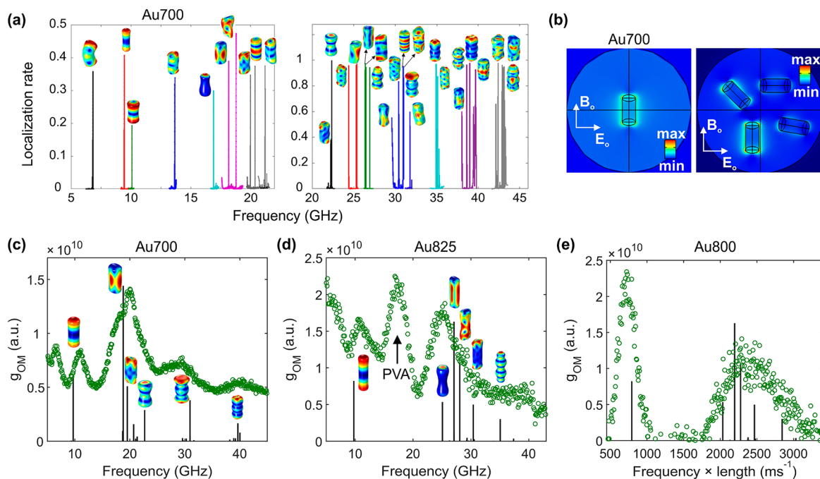
Figure 4. Eigenmodes, plasmons, and optomechanics of single Au NRs in PVA. (a) The localization rate as a function of the vibrational frequency revealing 32 eigenmodes of the Au700 monomer in PVA between 5 and 45 GHz. (b) The electric field distribution for a single Au700 NR with its long axis perpendicular to the incident electric field (left) and for a collection of Au700 NRs with different orientations (right). (c, d) The optomechanical coupling strengths (vertical bars) overlaid with the experimental BLS spectra (green dots) for comparison. The BLS active vibrational eigenmodes of Au700 and Au825 are shown as insets in (c) and (d), respectively. The strong peak at about 17 GHz in (b) is the effective medium longitudinal phonon in the polymer (PVA) matrix. (e) The optomechanical coupling spectrum for Au825 (vertical bars) overlaid with the BLS spectrum of the Au800 NRs (green dots) as a function of the frequency multiplied by the respective NR length. Au800 and Au825 NRs have very similar aspect ratios ( \alpha \approx 3.4 ).
