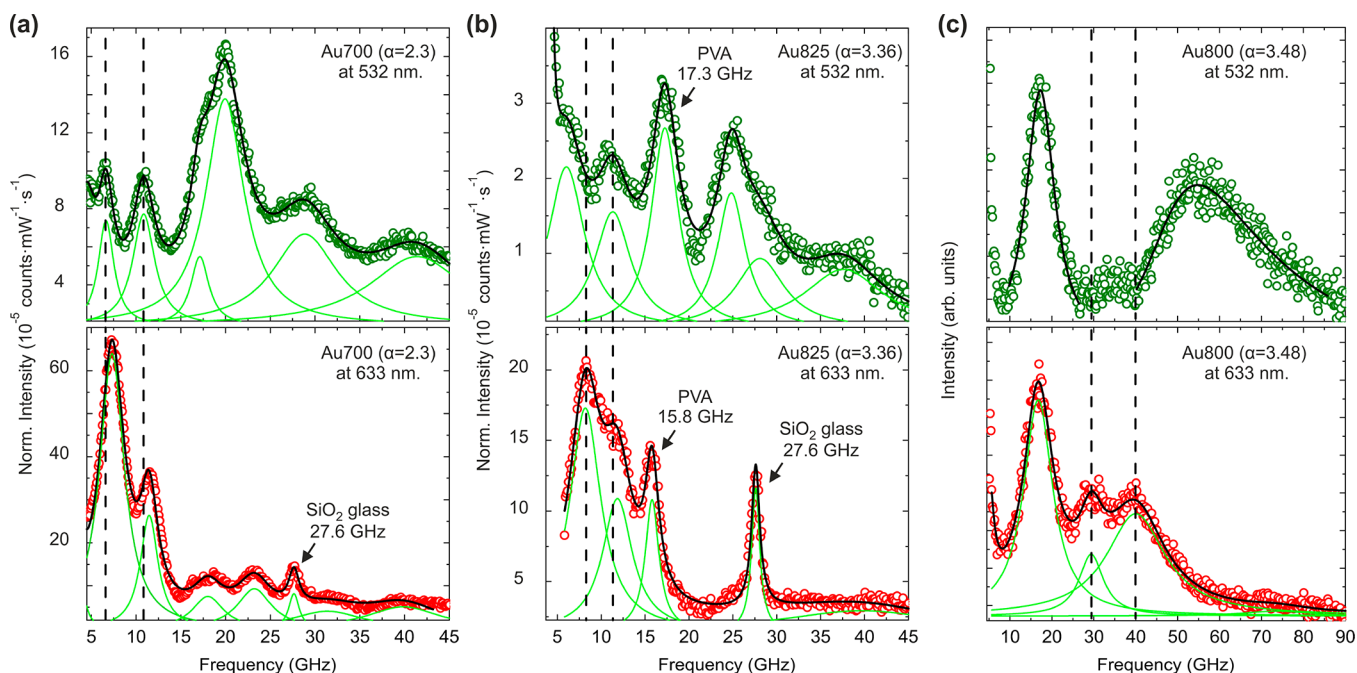
Figure 3. Wavelength-dependent inelastic light scattering spectra of Au NRs. (a–c) BLS spectra of Au700, Au825, and Au800 NRs with 532 nm (top) and 633 nm (bottom) CW light. The experimental data (points) are represented with a sum (solid black lines) of Lorentzian peak profiles (green lines). The measured BLS intensities have been normalized by the exposure time, the incident power, and the absorbance for Au700 and Au825, to quantify the plasmonic enhancement of the two lowest frequency modes.
