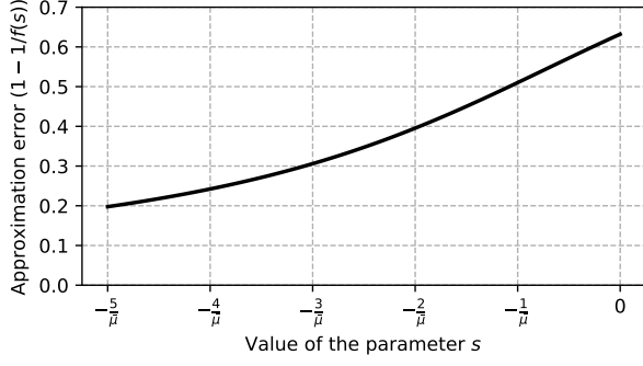
Figure 3. Values of the approximation error (1 - 1/f(s)) provided in the bound of Proposition 4.3 for different values of s .
