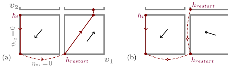
Fig. 5: Illustration of blockage (a) and wrong discrete transition (b).
