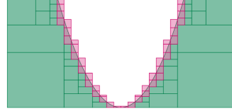
Fig. 3: CSP difficulty to target solutions for constraint y \leq x^2 .
