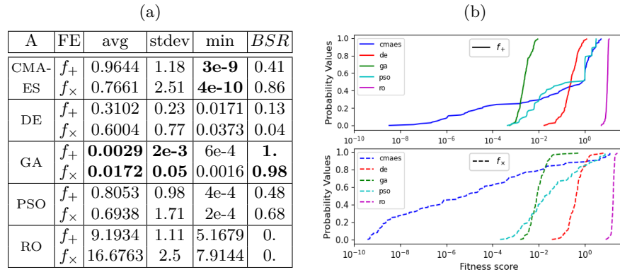
Fig. 7: Summary (a) and CDF curves (b) of overall best results.
