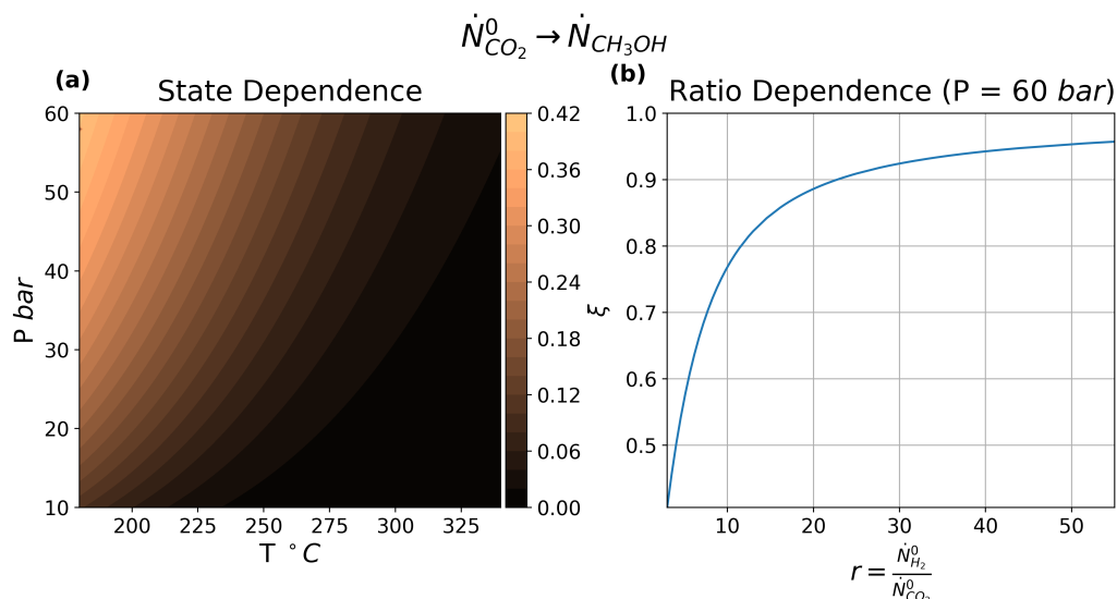
Figure 9. The conversion factor, \zeta , or the percentage of moles of CO_2 transformed into CH_3OH . It was calculated using the equilibrium equations presented in Terreni et al., 2020 [33], with varying state conditions ( P and T ) and molar ratios of H_2 and CO_2 . The state dependence curve was calculated with a H_2/CO_2 molar ratio of 3, which is the stoichiometric ratio. Subplot (a) shows \zeta 's dependency on pressure and temperature. (b) shows \zeta 's dependency on the input ratio of H_2 and CO_2 .
