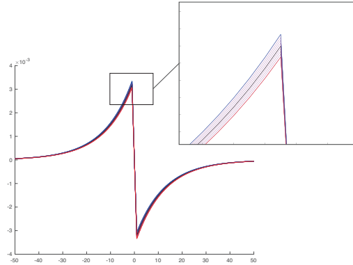
Fig. 2: \bar{\psi} (in blue), \psi (in red), 8 impulse responses for different kernels within the family represented by \pi (in magenta), and the response of the Dirac kernel (in black).
